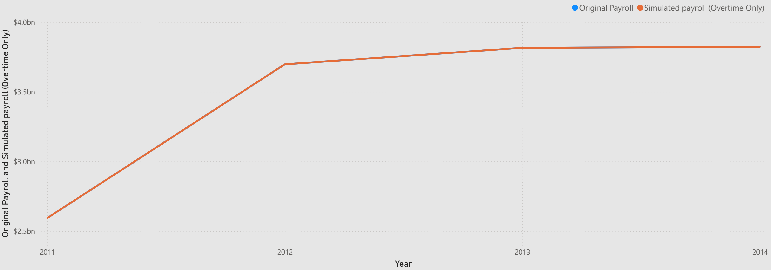
Original vs Simulated Payroll by Year
