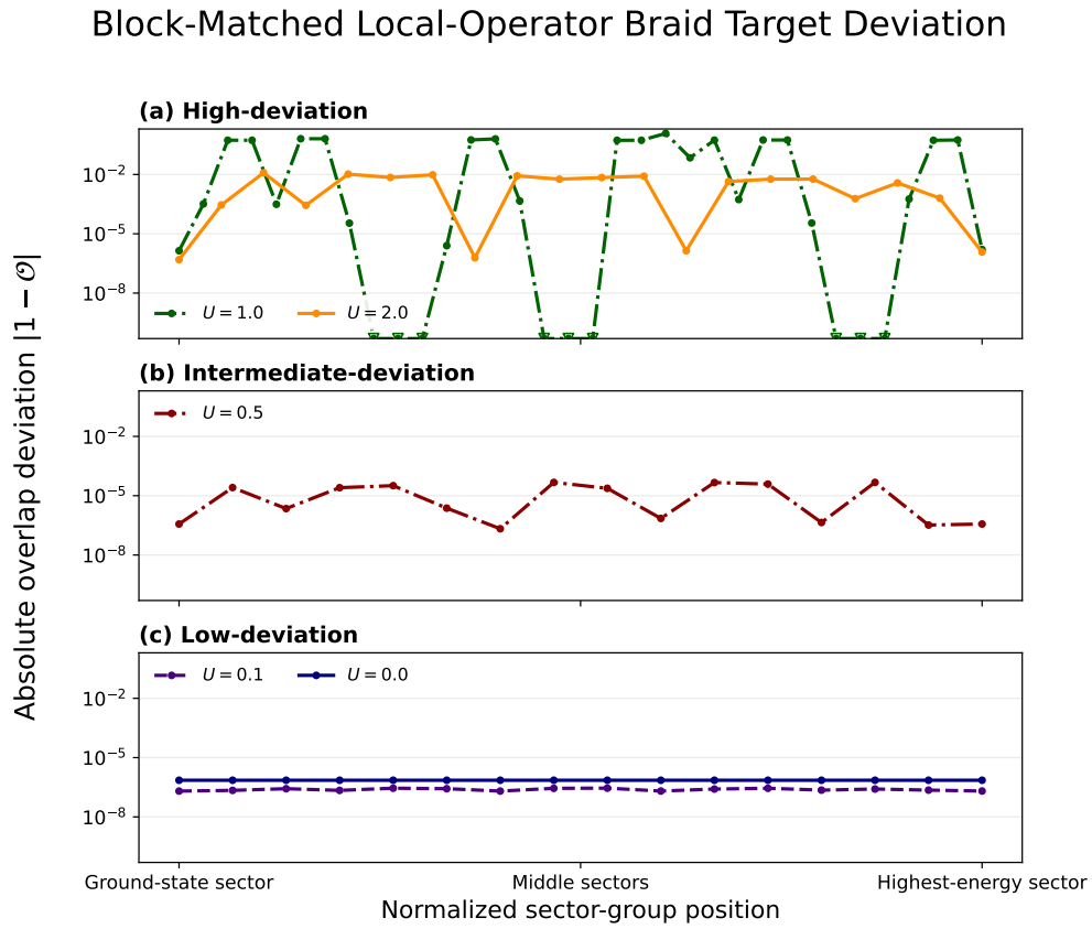
Figure 4.14: Self-target braid errors for the block-matched local-operator model, plotted as the overlap deviation D_{\mathcal{O}} = |1 - \mathcal{O}| . The same three deviation regimes as in Fig. 4.12 remain visible: a) U = 1.0 and U = 2.0 , b) U = 0.5 , and c) U = 0.0 and U = 0.1 .
