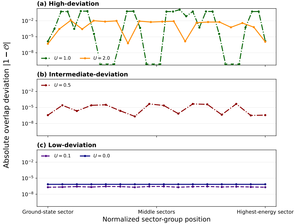
Figure 4.12: Self-target braid errors for the projected local-operator model across different energy sectors and interaction strengths U = 0.0 , U = 0.1 , U = 0.5 , U = 1.0 , and U = 2.0 , plotted as the overlap deviation D_{\mathcal{O}} = |1 - \mathcal{O}| . The figure is split into three deviation regimes: a) U = 1.0 and U = 2.0 , b) U = 0.5 , and c) U = 0.0 and U = 0.1 . The selected weak-interaction configurations have low deviations across all sectors, while the selected stronger-interaction configurations contain sectors with larger self-target errors.
