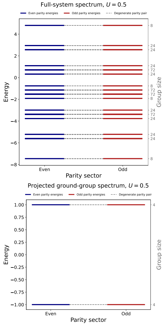
Figure B.3: Energy spectrum and ground state splitting after Hamiltonian initiation. System configuration and optimization results are reported in Table 4.1. These figures are for the U = 0.5 configurations, for the three identical three dot systems.
