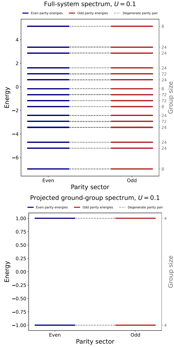
Figure B.2: Energy spectrum and ground state splitting after Hamiltonian initiation. System configuration and optimization results are reported in Table 4.1. These figures are for the U = 0.1 configurations, for the three identical three dot systems.
