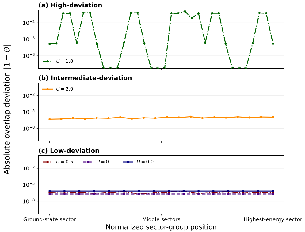
Figure 4.11: Self-target braid errors for the energy-level Majorana baseline across different energy sectors and interaction strengths U = 0.0 , U = 0.1 , U = 0.5 , U = 1.0 , and U = 2.0 , plotted as the overlap deviation D_{\mathcal{O}} = |1 - \mathcal{O}| . The figure is split into three deviation regimes: a) U = 1.0 , b) U = 2.0 , and c) U = 0.0 , U = 0.1 , and U = 0.5 . The energy-level construction supports accurate braiding across all sectors for the non-interacting and weakly interacting configurations, while the U = 1.0 configuration shows strong sector-dependent failures.
