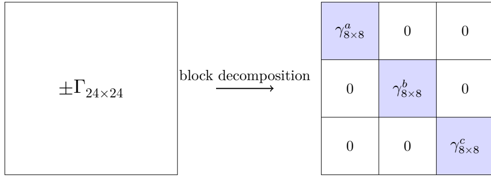
Figure 4.13: Schematic decomposition of a projected local Majorana operator in a 24-dimensional energy sector. The sector separates into three independent 8 \times 8 blocks, labelled a , b , and c , with one effective Majorana block acting within each subspace.
