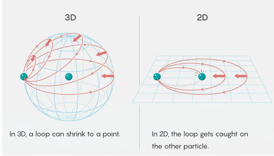
Figure 2.1: Visualization of particle exchange in two and three dimensions. Illustration by 5W Infographics for Quanta Magazine, reproduced from [28].
