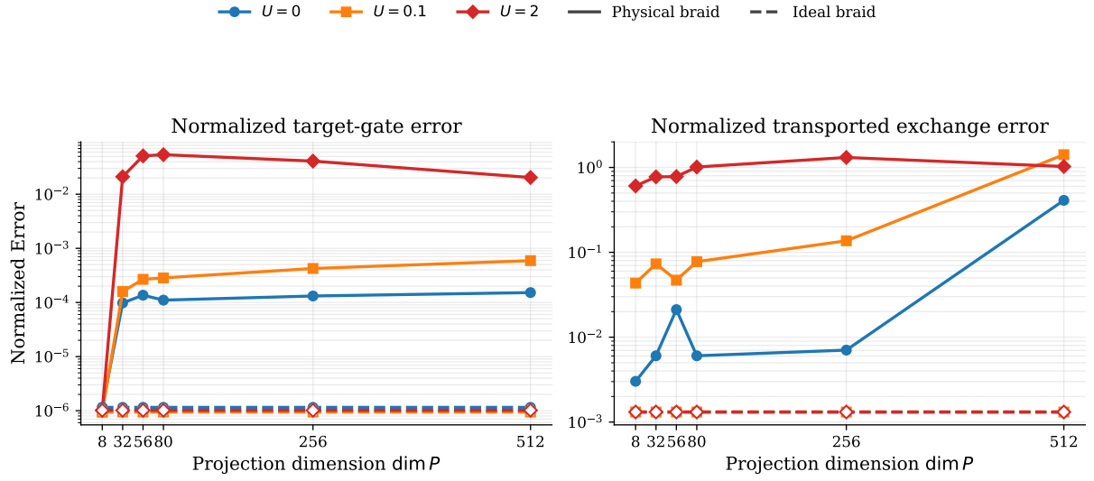
Figure 20: The same interaction comparison extended to \dim P = 256 and 512 . The full-range plot documents the high-dimensional endpoints used in Table 5. The noninteracting target-gate error remains small even at the largest projection sizes, but the physical-versus-ideal diagnostics in the companion plots reveal that high-dimensional projected spaces can still expose basis mismatch in the microscopic junction description.
