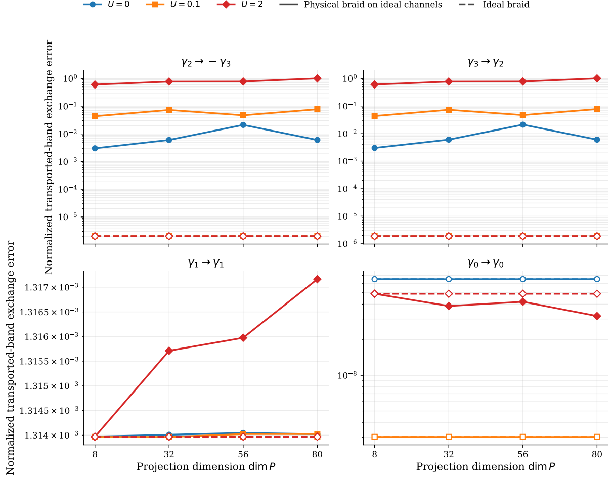
Figure 19: Transported-band channel-resolved exchange errors for \dim P \leq 80 . Unlike the earlier full-projection operator diagnostic, this plot evaluates V^\dagger(U^\dagger \gamma_i U - \gamma_j)V inside the transported band V . The exchanged channels therefore agree with the target-gate diagnostics: U = 0 remains close to the ideal exchange, U = 0.1 gives an intermediate deviation, and U = 2 fails primarily in the intended exchange channels.
