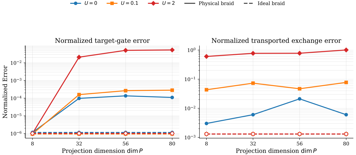
Figure 17: Interaction comparison for the corrected minus-channel projection scan, restricted to \dim P \leq 80 . The left panel shows the normalized target-gate error, while the right panel shows the transported-band exchange error on the ideal Majorana channels. The dashed ideal curves are control calculations and remain near the numerical integration floor. The physical curves show the expected separation: U = 0 stays small, U = 0.1 is slightly worse, and U = 2 is strongly degraded once excited sectors enter.
