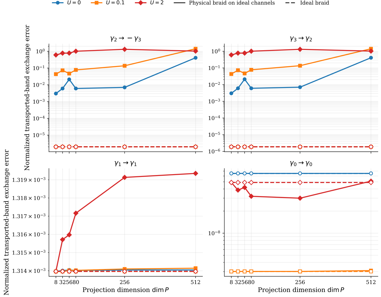
Figure 21: Transported-band channel-resolved exchange errors for the full \dim P \leq 512 scan. The high-dimensional endpoints preserve the same qualitative hierarchy: the ideal control remains accurate, the weakly interacting case is intermediate, and the strongly interacting case has order-one exchange-channel mismatch. The extended scan is mainly a robustness check; the \dim P \leq 80 window remains easier to interpret visually.
