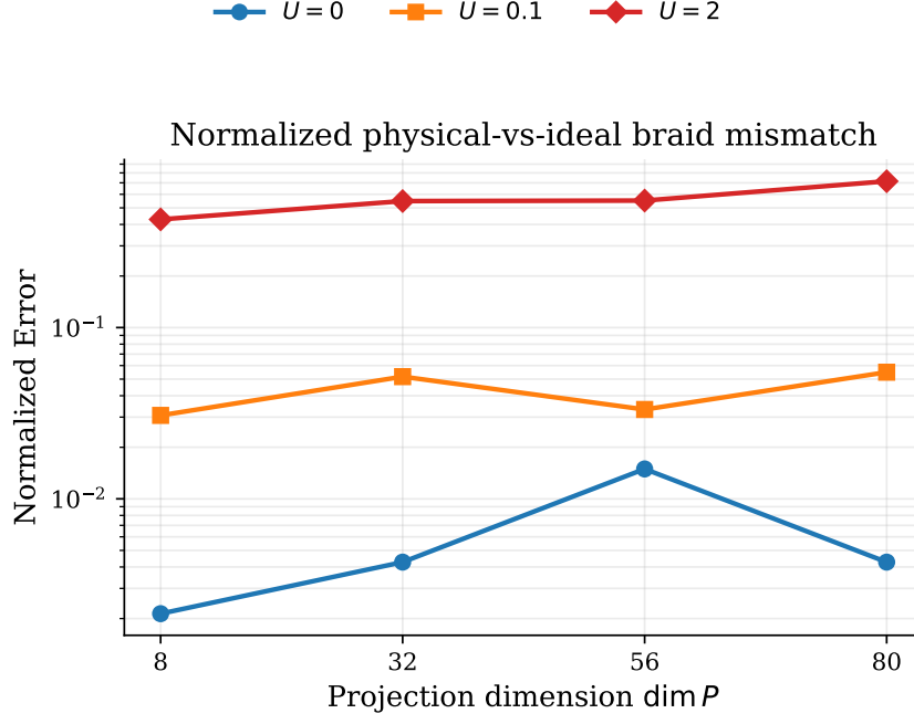
Figure 18: Direct physical-versus-ideal braid mismatch for \dim P \leq 80 . This is the cleanest diagnostic of whether the microscopic minus-channel junction implements the same braid as the ideal projected-Majorana Hamiltonian. The weakly interacting case remains close to the noninteracting result, while the U = 2 mismatch is already large at the first excited projections.
