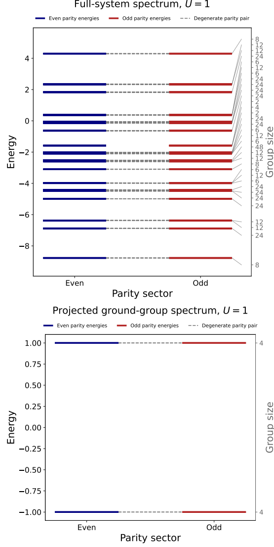
Figure B.4: Energy spectra and ground state splitting after Hamiltonian initiation. System configuration and optimization results are reported in Table 4.1. These figures are for mode U = 1.0 , for the three identical three dot systems. This plot also reflects the braiding results of U = 1.0 , as both the braiding and these energy sectors are chaotically unstable.
