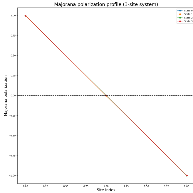
Figure 11: The two plots show the parity resolved spectrum after optimization for the three dot system, with interaction strength U = 0.1 . The optimized parameters are shown schematically below the left plot, and the Majorana polarization profile of the lowest-energy states is shown in the right plot.
