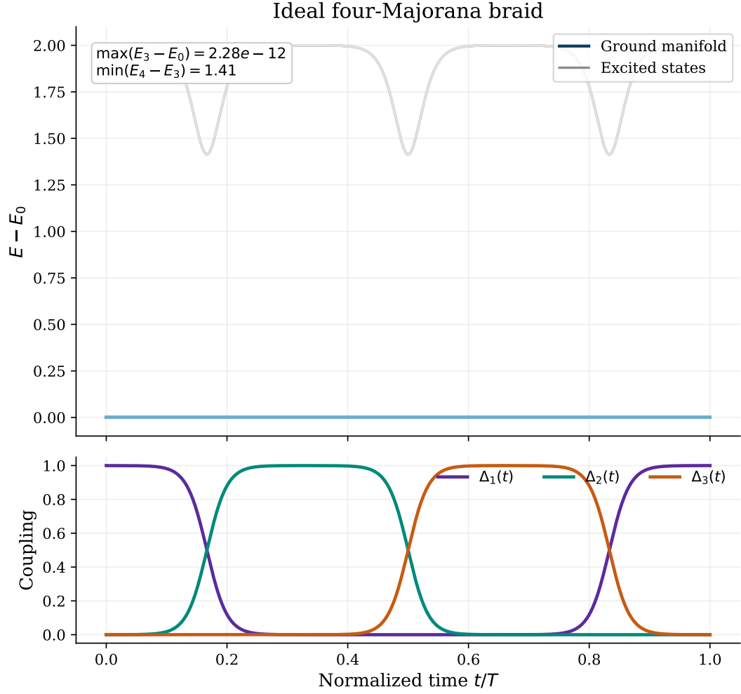
Figure 15: Idealized four-Majorana braiding protocol. The top panel shows the instantaneous spectrum of the effective Hamiltonian during the braid, with all energies shifted so that the lowest state remains at zero. The bottom panel shows the three smooth pulse couplings that move the dominant Majorana pairing through the network.
