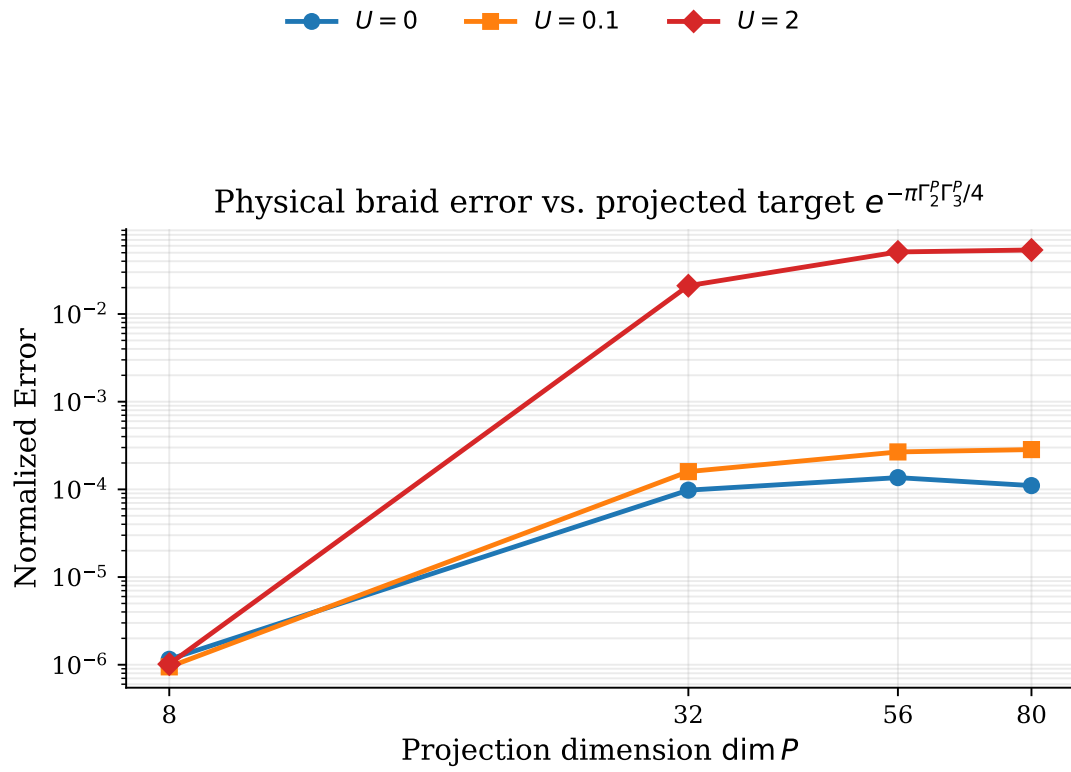
Figure 19: Local-operator braid error up to \dim P = 80 . Here the braid is generated and judged using the projected local endpoint operators Pi(c^\dagger - c)P . This is the more microscopic diagnostic, because it tests how well the exchange channel is accessed by a local physical coupling.
