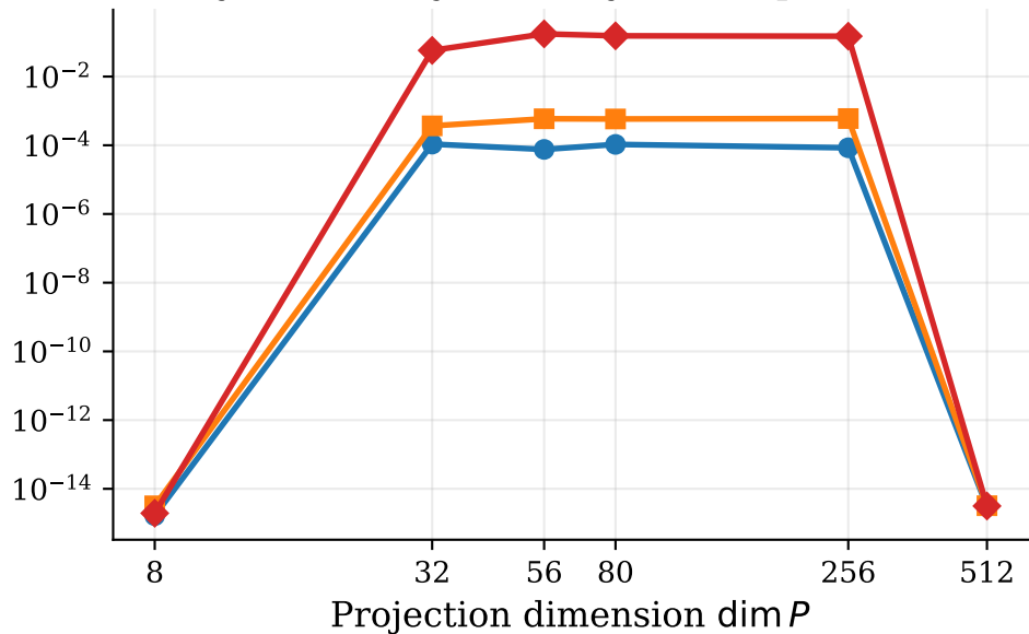
Projected analytical Majorana square error
