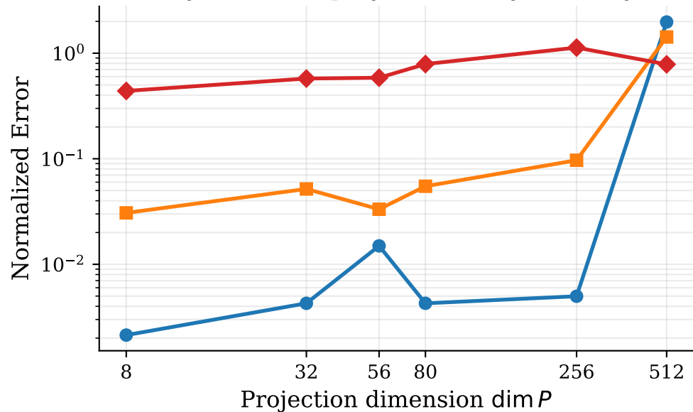
State Majoranas vs. projected analytical Majoranas
