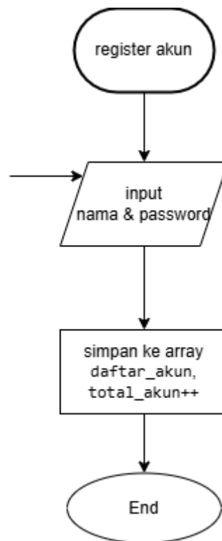
Gambar 2.4 Flowchart Register Akun Menu 1
