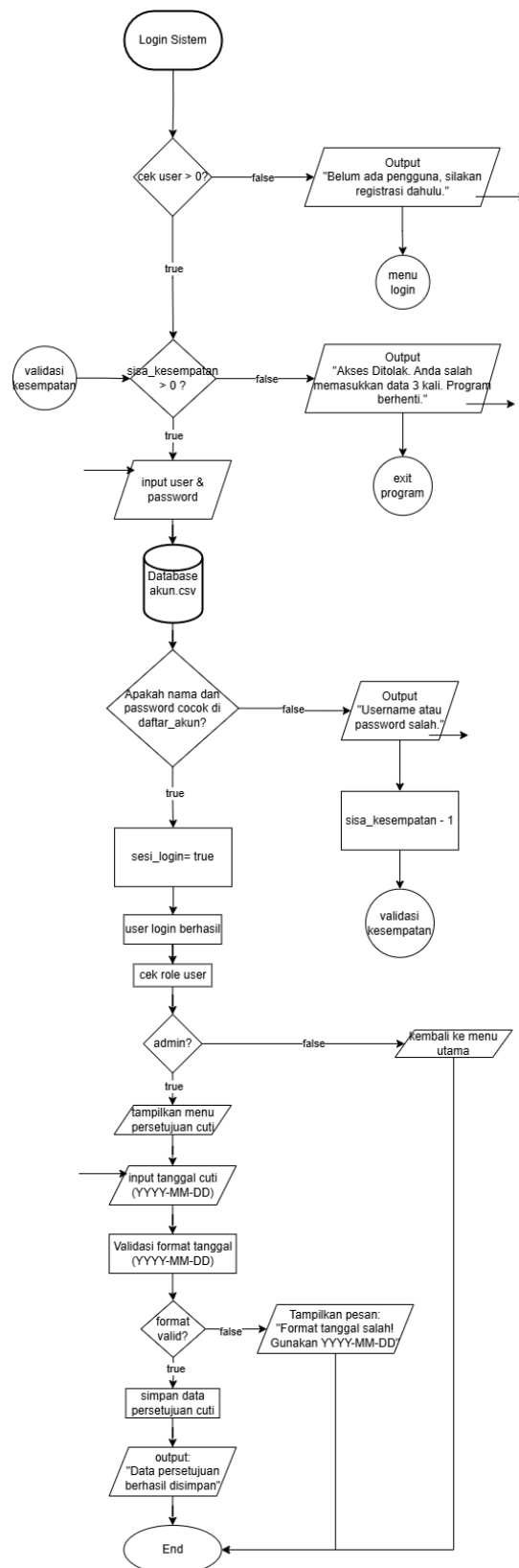
Gambar 2.2 Flowchart Login Sistem
