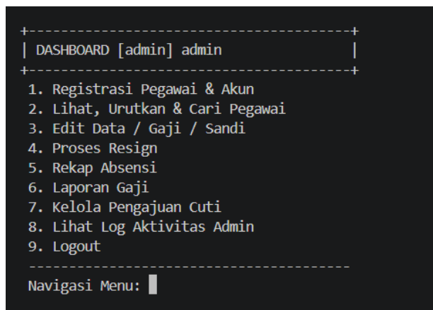
Gambar 3.3 Output Menu Admin
