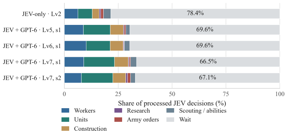
(a) Action allocation (wait share labeled)
