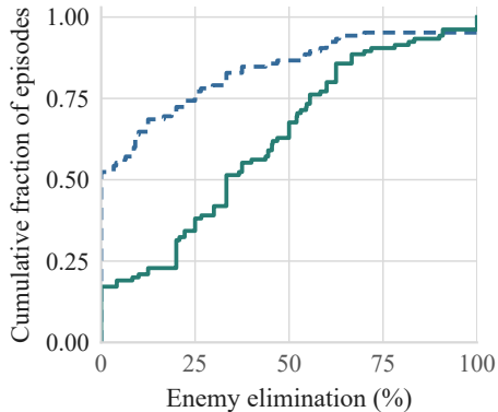
(a) All 105 episodes per method
