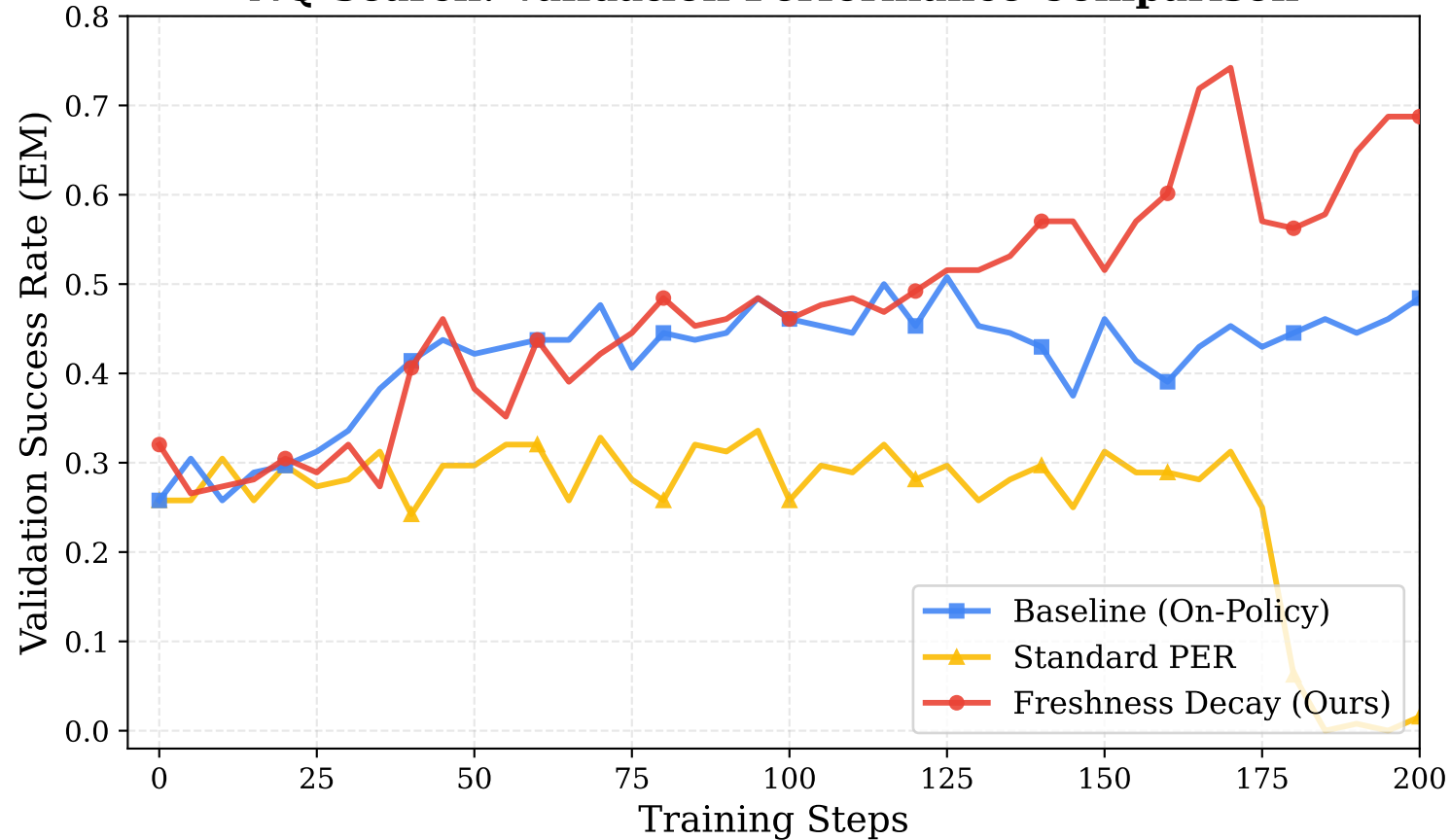
NQ Search: Validation Performance Comparison
