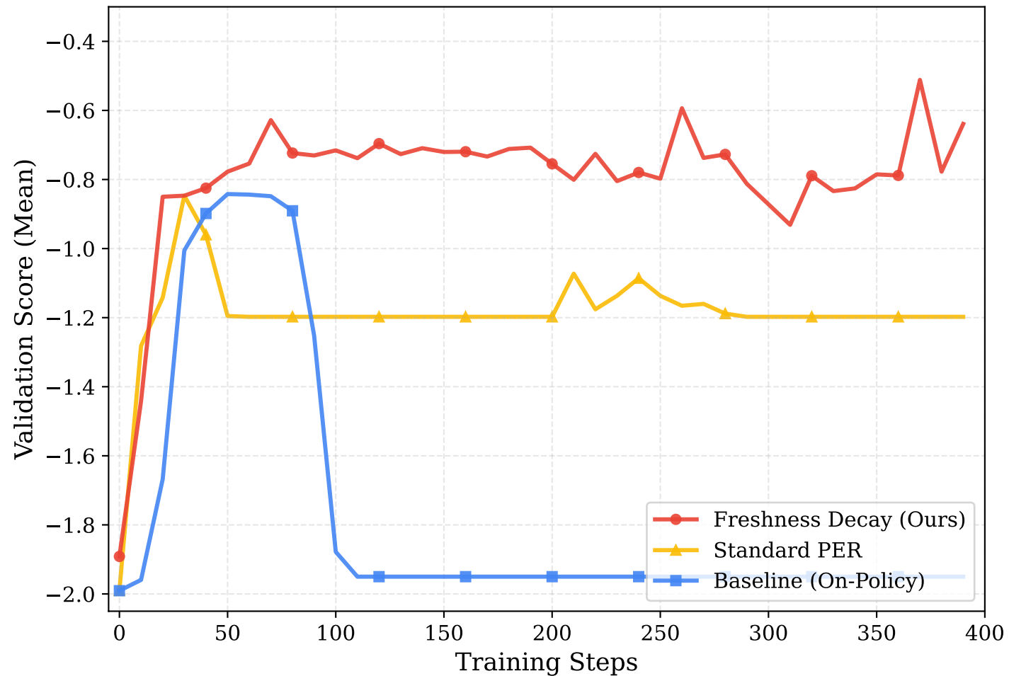
Sokoban Hard: Validation Score
