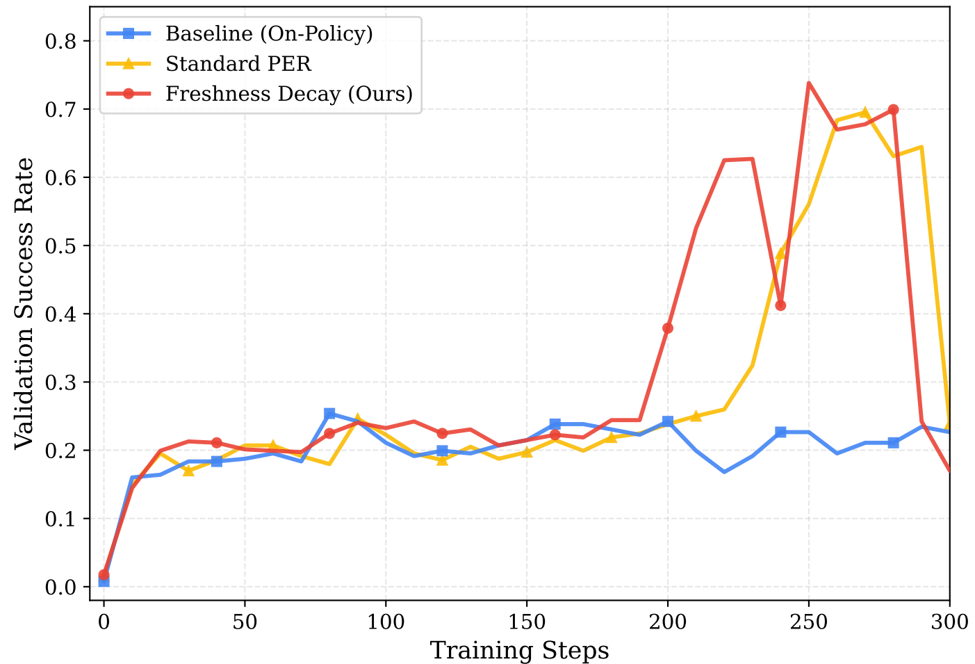
VLM FrozenLake: Validation Success Rate
