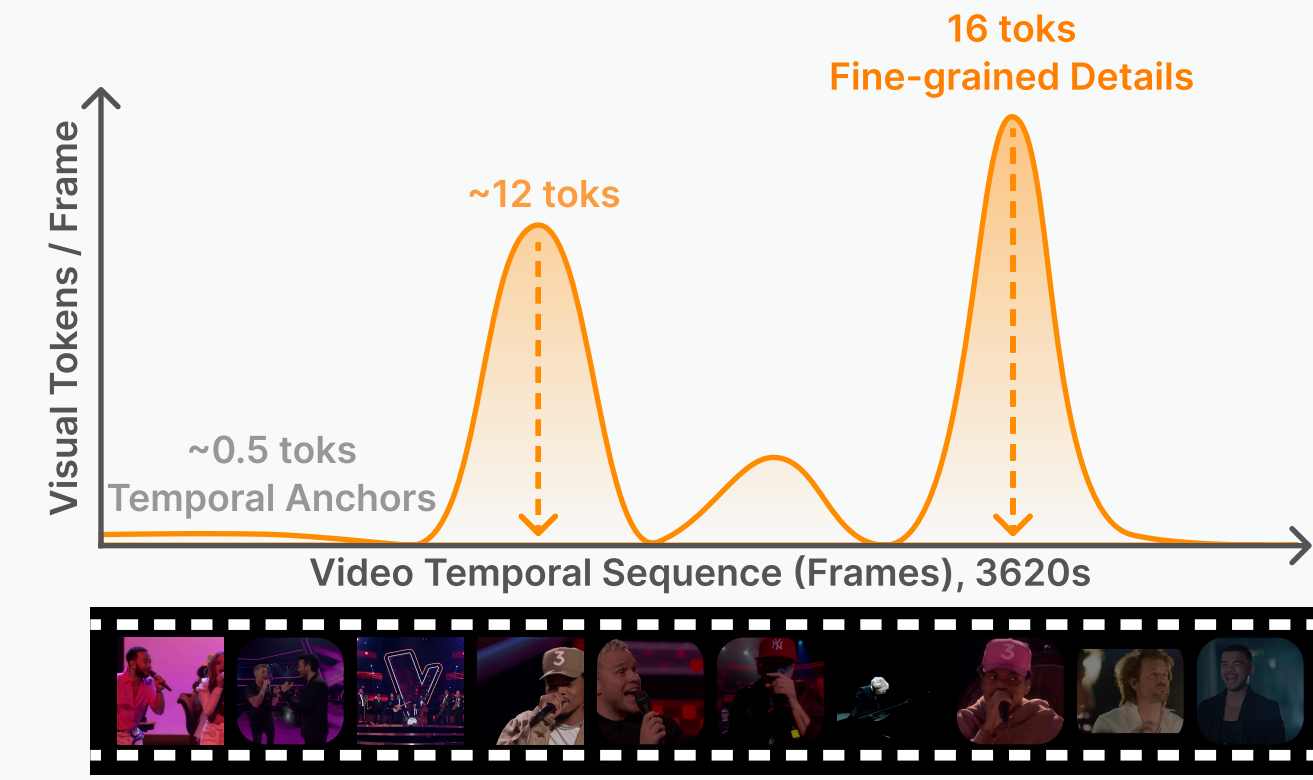
(b) Mechanism: Adaptive Token Allocation (ATA) visualized over time
