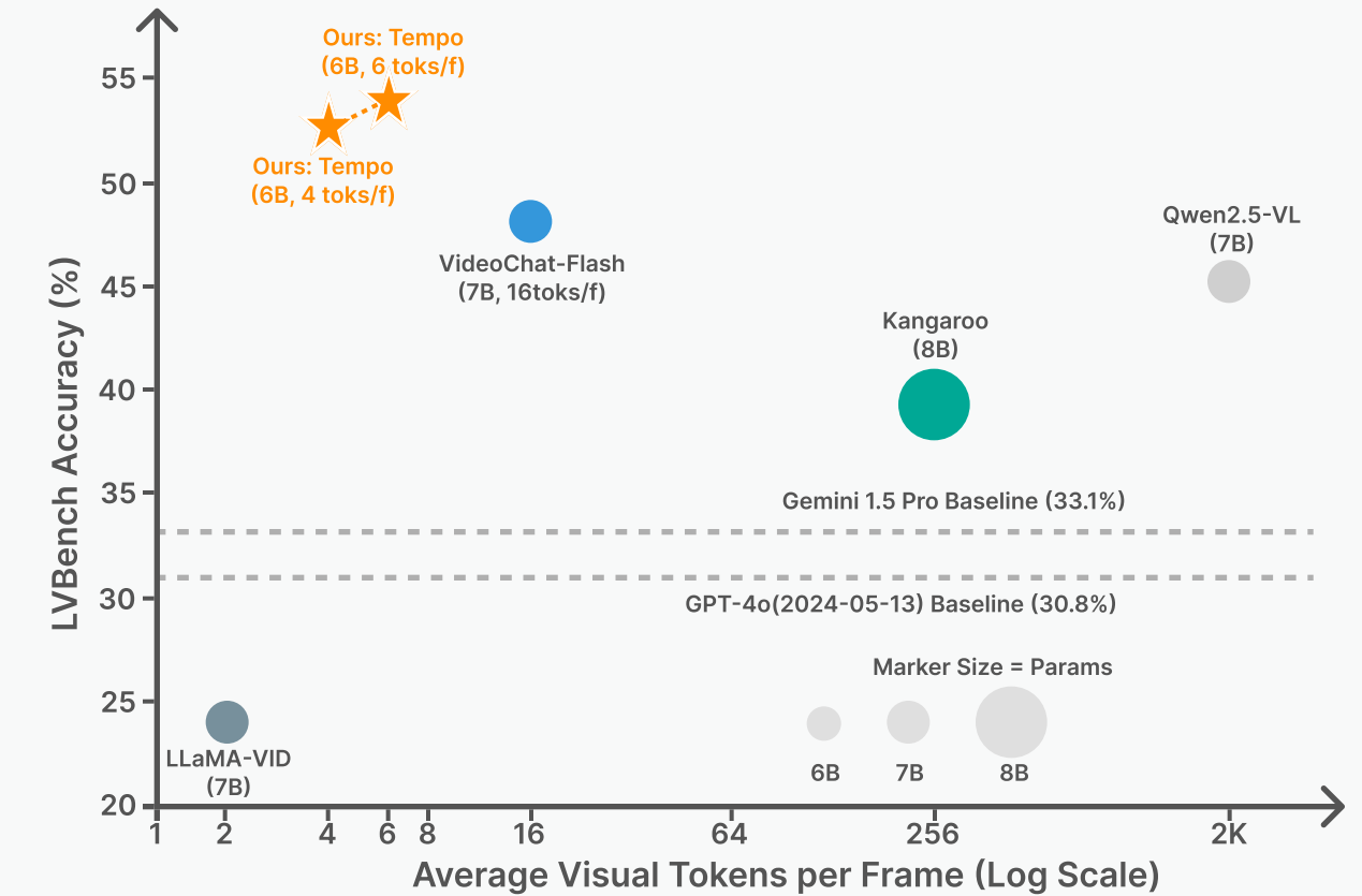
(c) Result: Efficiency vs. Performance (LVBench)
