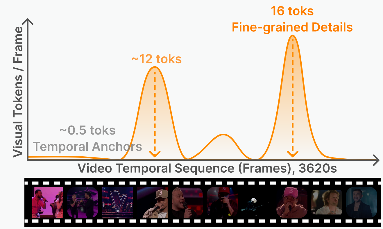
(b) Adaptive Token Allocation visualized over time
