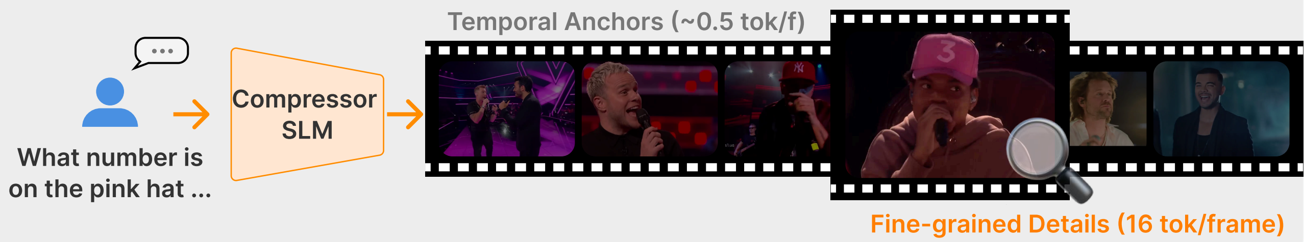
(a) Existing Query-Agnostic Methods vs. Ours (Query-Aware)
