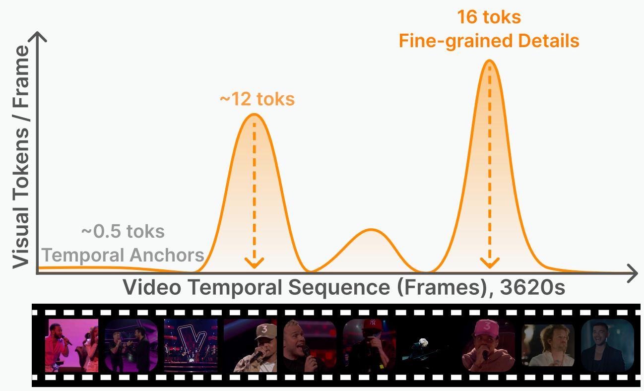
(b) Adaptive Token Allocation visualized over time
