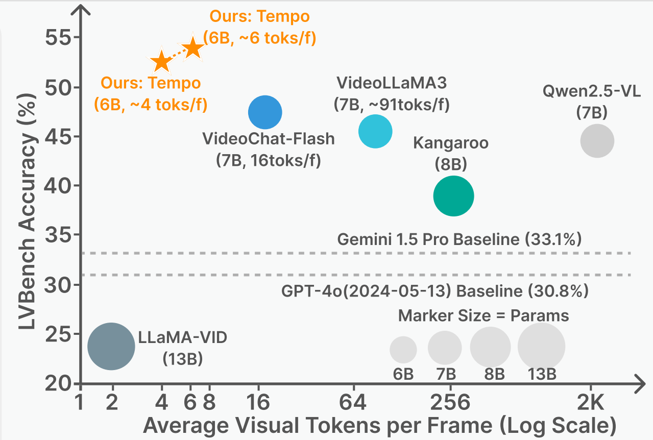
(c) Efficiency vs. Performance (LVBench)
