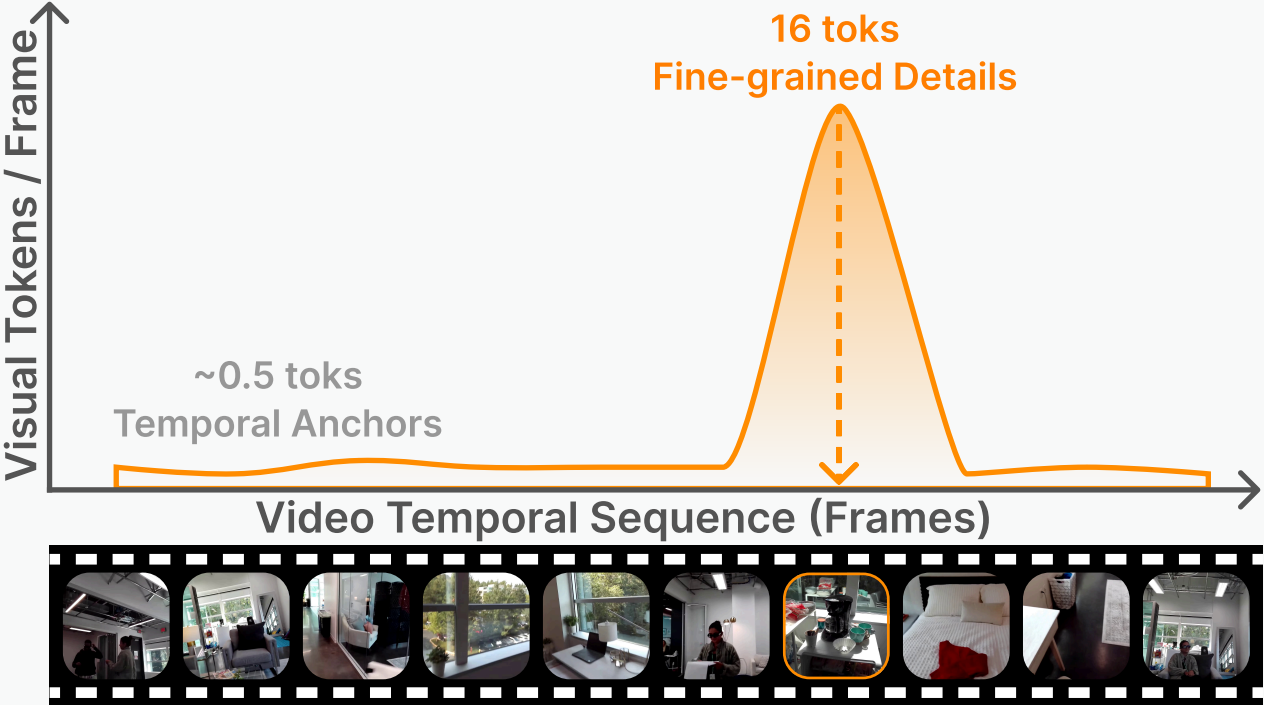
(b) Adaptive Token Allocation Visualized over Time
