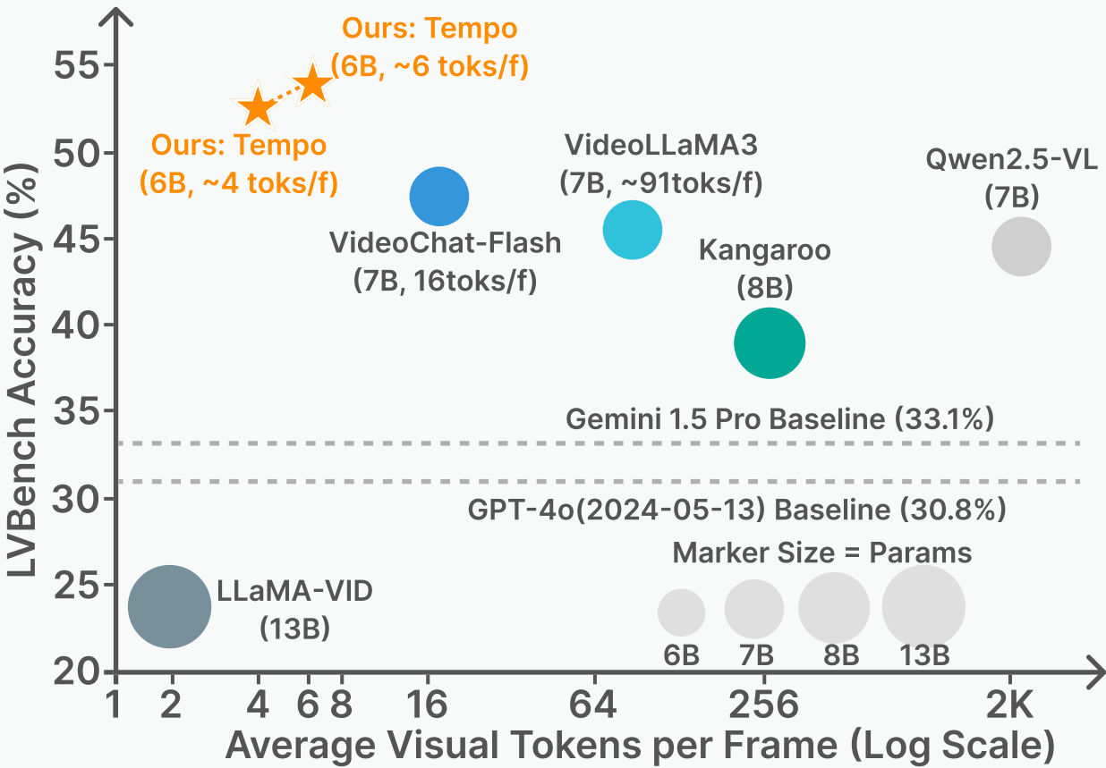
(c) Efficiency vs. Performance (LVBench)
