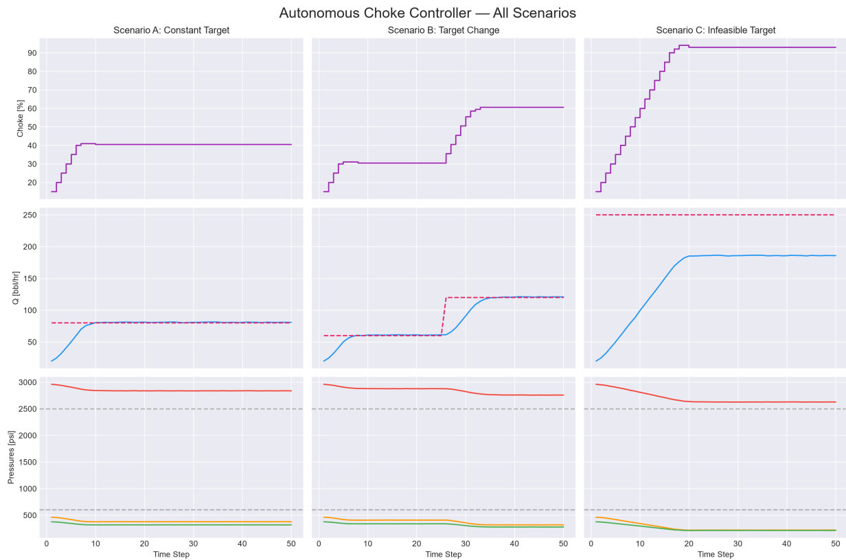
Figure 4: Summary dashboard: All 3 scenarios side-by-side comparison.
