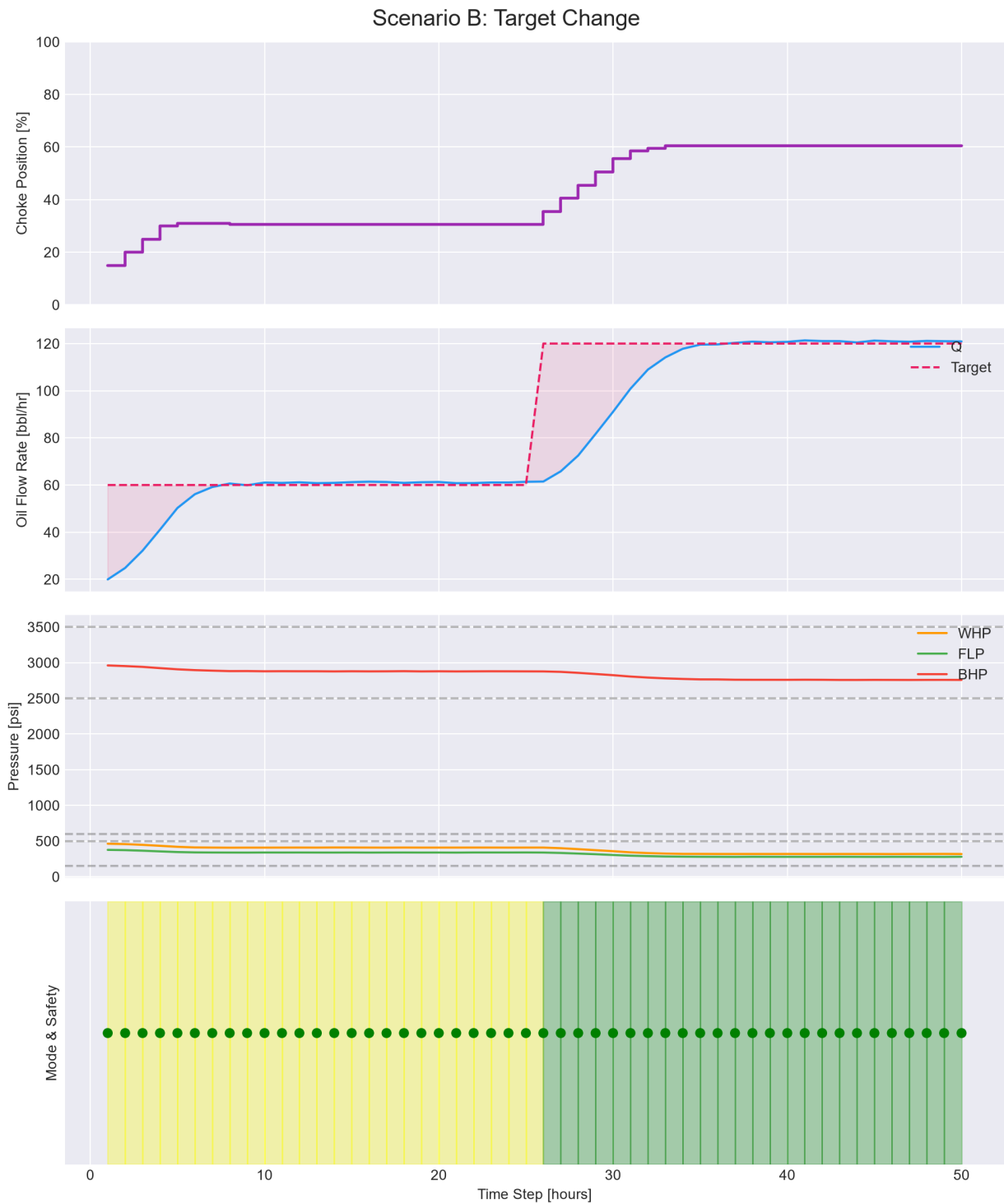
Figure 2: Scenario B: Setpoint transition. Smooth ramp, TRACKING mode, 0 violations.
