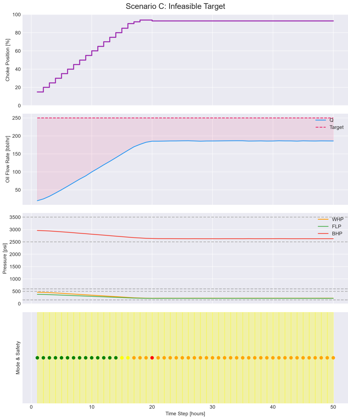
Figure 3: Scenario C: Constraint-limited max production. Choke at 93%, Q=186 bbl/hr.
