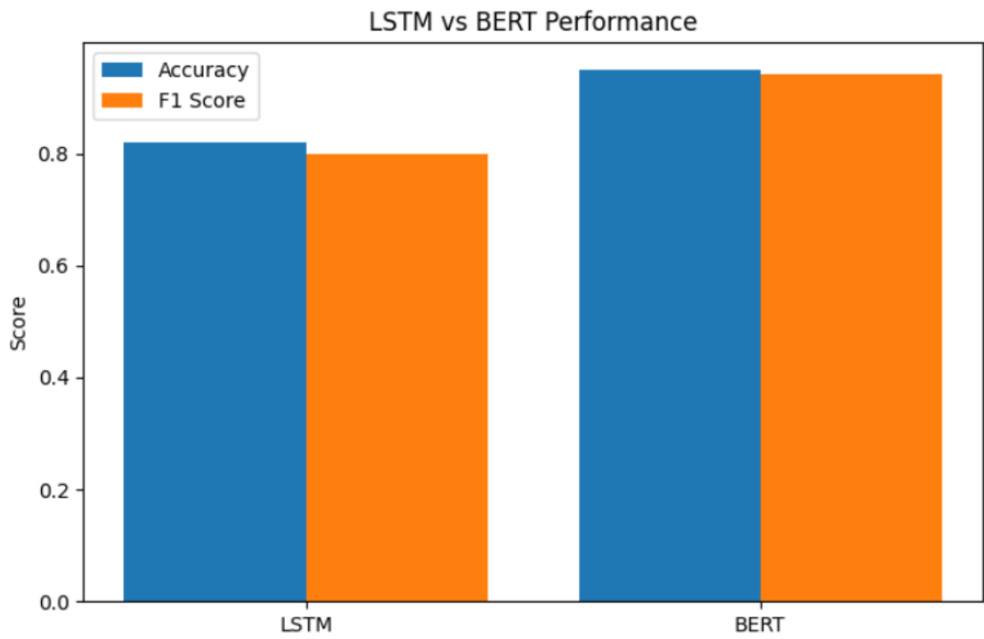
Figure 2 Accuracy and F1 score, LSTM vs BERT
