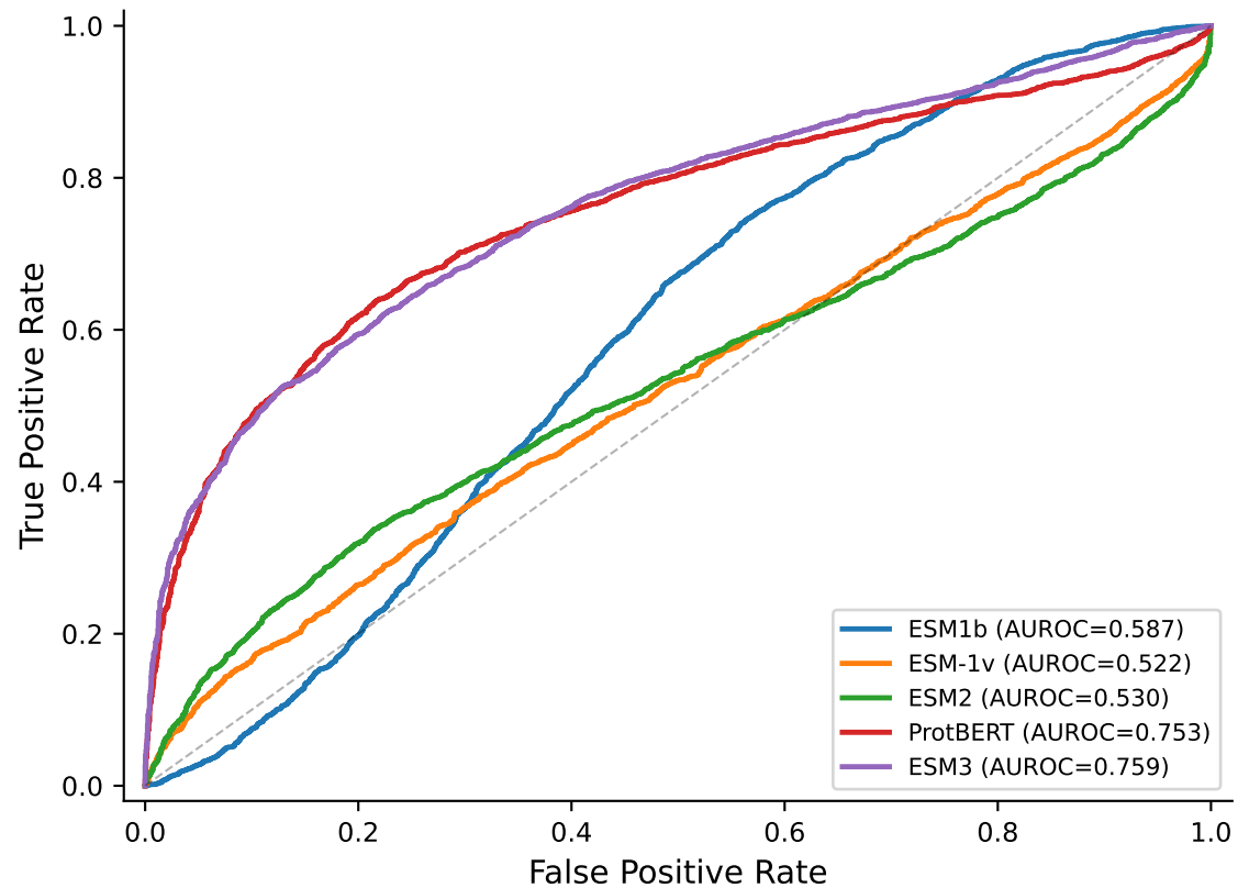
B. Cosine Distance (All Models)
