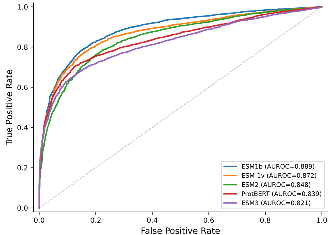
A. MLM Scoring (Top Models)
