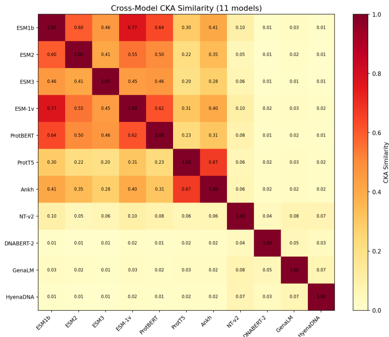
Figure 6: Cross-model CKA similarity matrix (median-heuristic RBF kernel). Protein models form a high-similarity cluster (upper-left), while nucleotide models are nearly orthogonal. Cross-modality CKA never exceeds 0.104.
