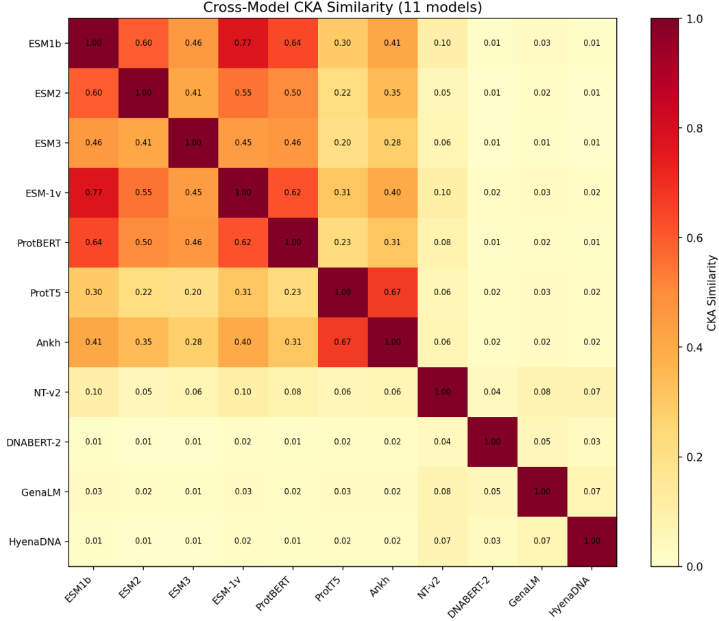
Figure 8: Full 11 \times 11 cross-model CKA matrix (median-heuristic RBF kernel). Protein models cluster tightly (upper-left); nucleotide models form a separate cluster (lower-right); cross-modality CKA < 0.104 .
