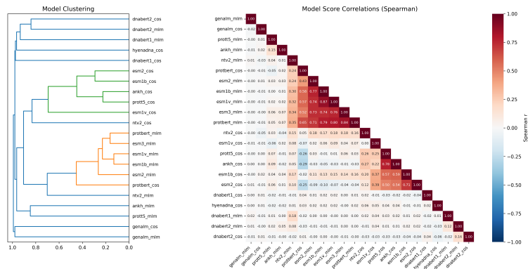
Figure 1: Pairwise Spearman correlation. Protein MLM models are highly correlated ( r = 0.68\text{--}0.83 ). Nucleotide models are nearly orthogonal to protein models ( r \approx 0.00 ).
