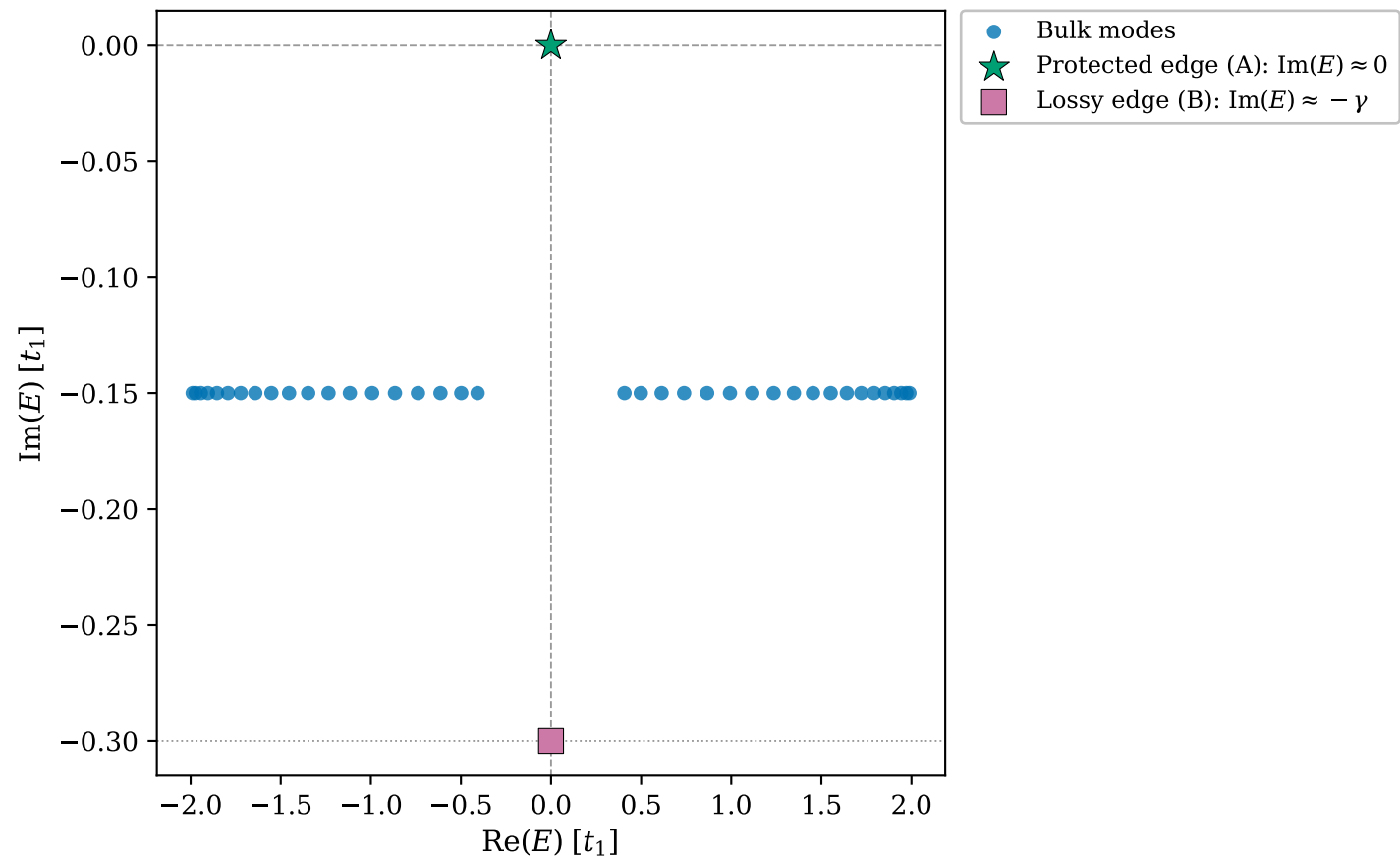
Complex spectrum — non-Hermitian SSH ( N = 20 , \gamma = 0.3 t_1 )
