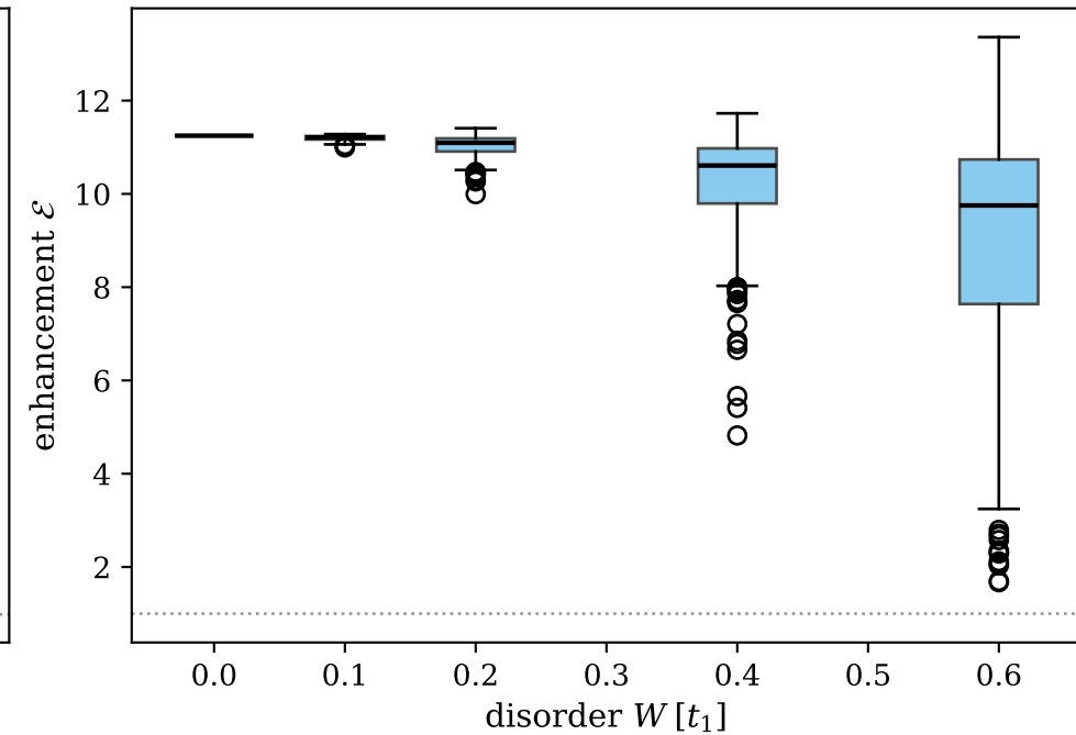
On-site \varepsilon distribution (200 realisations)
