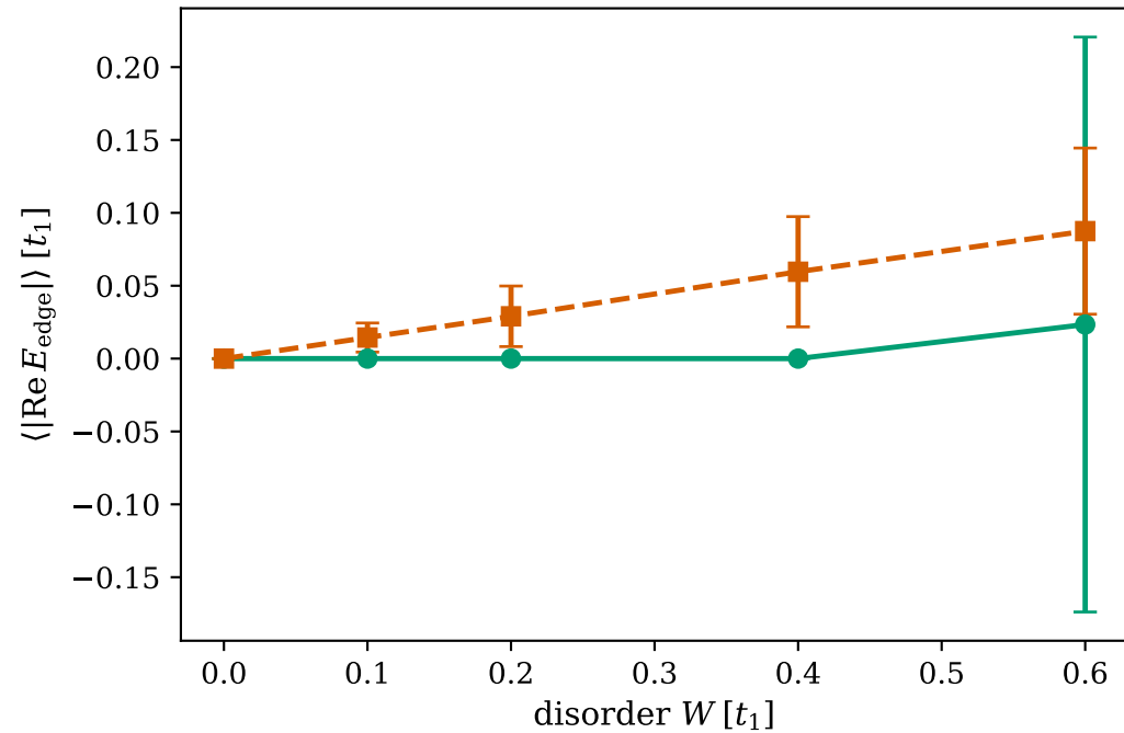
Zero-mode pinning (protection diagnostic)
