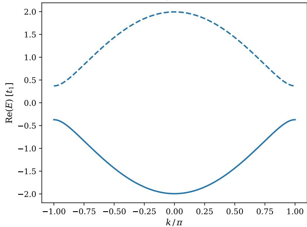
Bloch Band Dispersion (Real Part)
