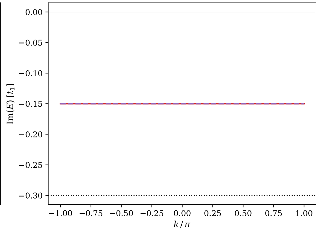
Bloch Band Decay Rates (Imaginary Part)
