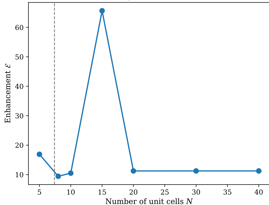
Finite-Size Convergence of LDOS Enhancement
