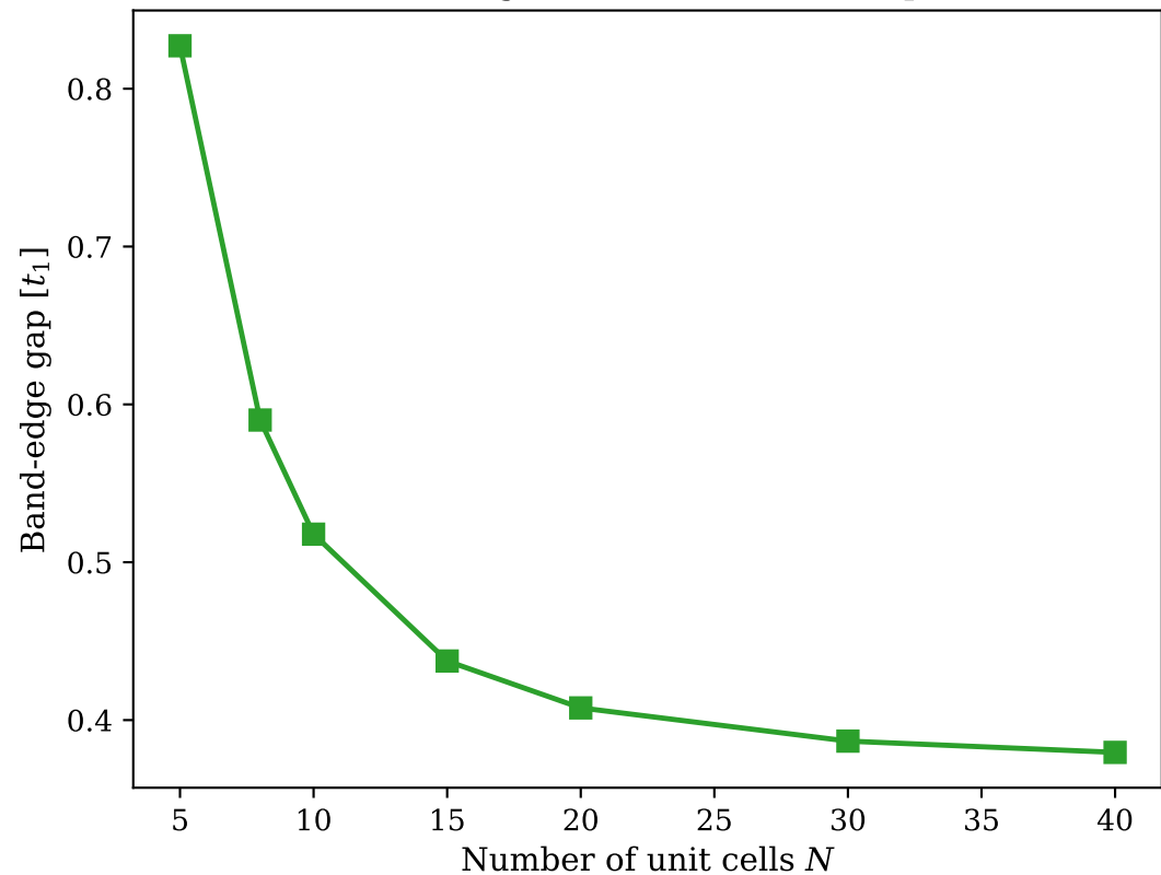
Convergence of OBC Band Gap
