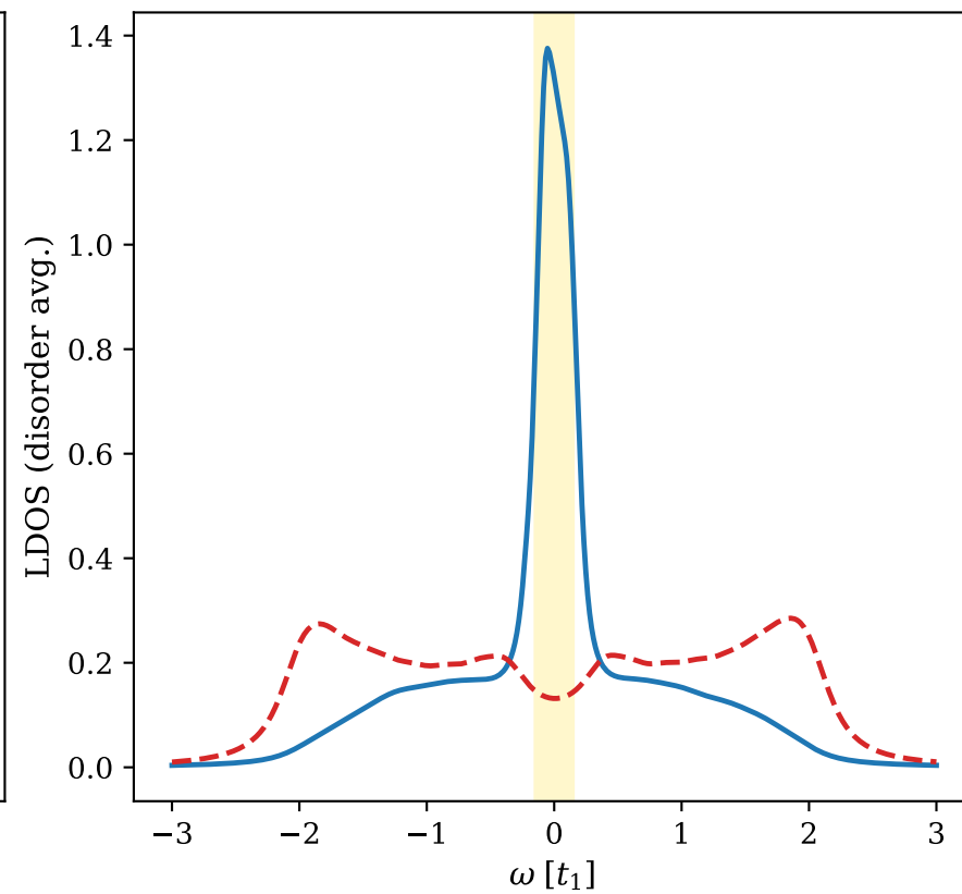
W = 0.6 t_1 - \langle \mathcal{E} \rangle = 8.9
