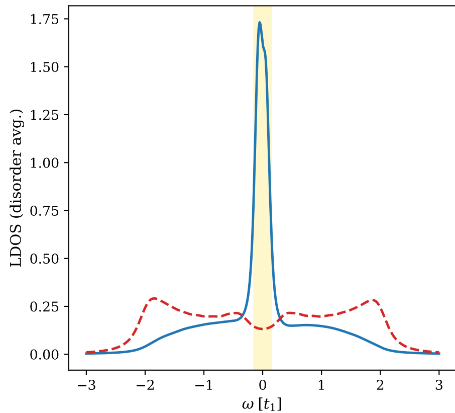
W = 0.4 t_1 - \langle \mathcal{E} \rangle = 10.1
