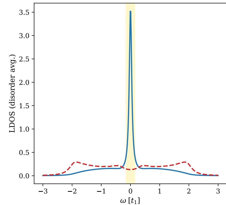
W = 0.0 t_1 - \langle \mathcal{E} \rangle = 11.2
