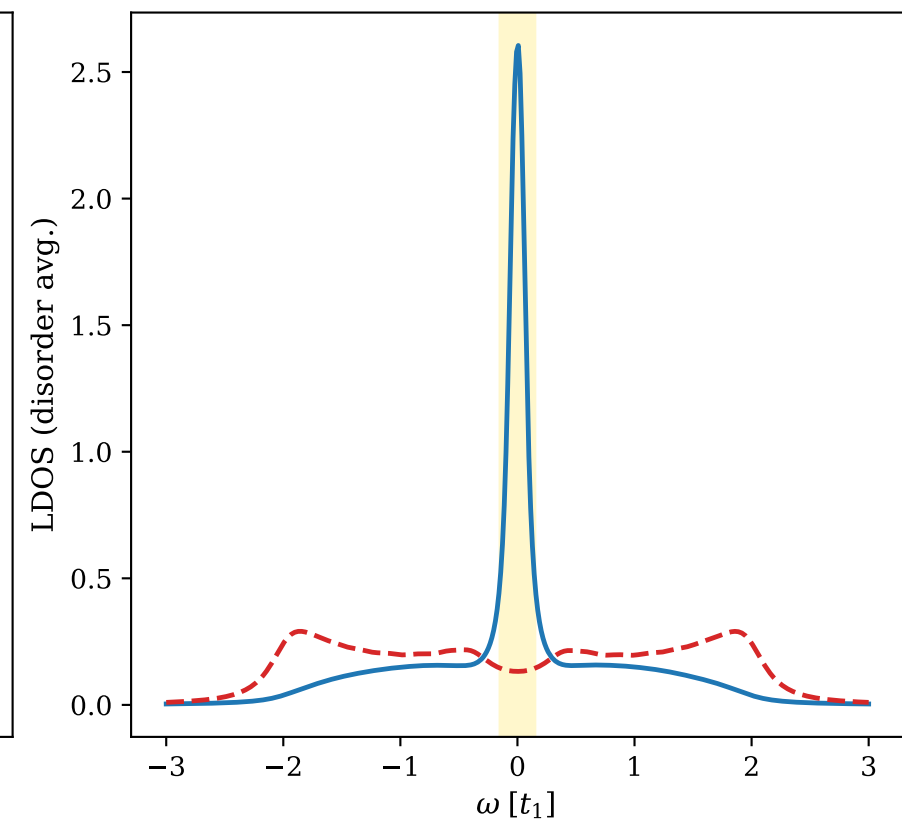
W = 0.2 t_1 - \langle \mathcal{E} \rangle = 11.0
