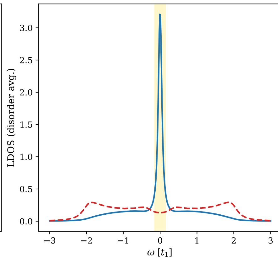
W = 0.1 t_1 - \langle \mathcal{E} \rangle = 11.2
