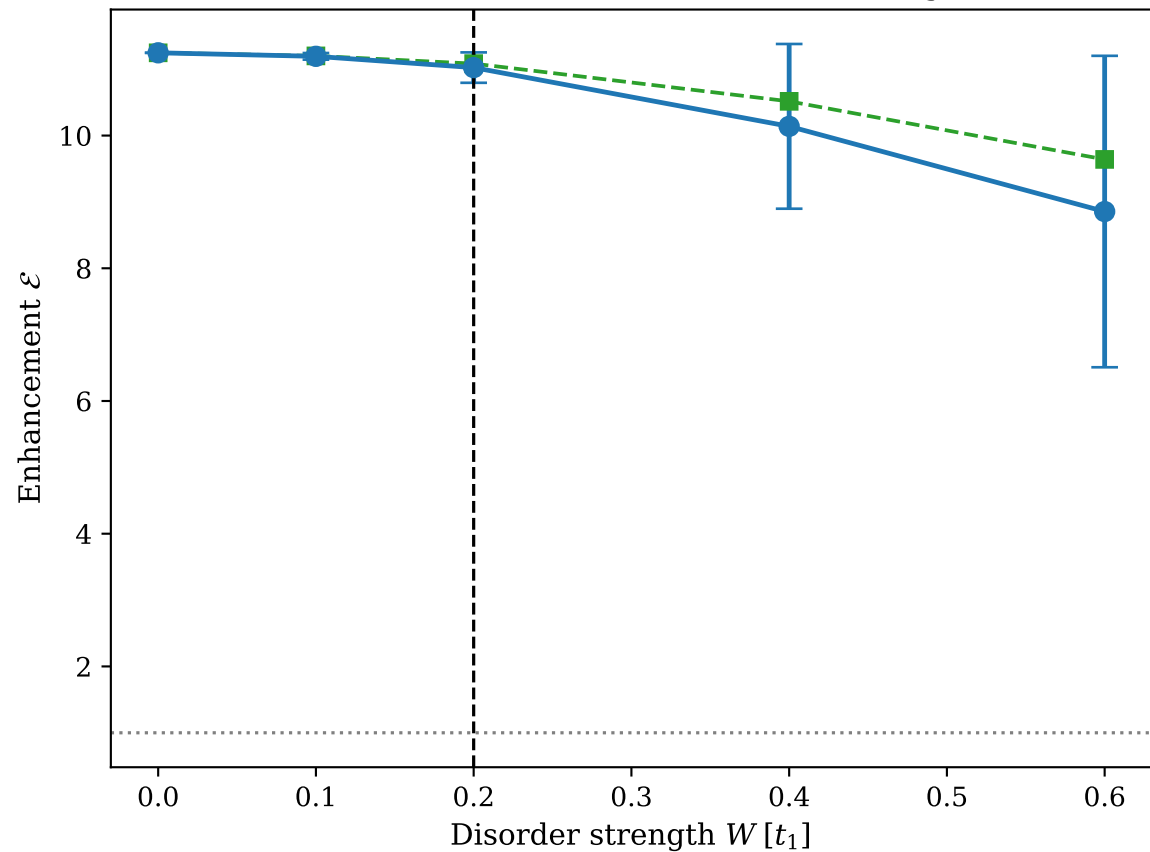
LDOS Enhancement vs. Disorder Strength
