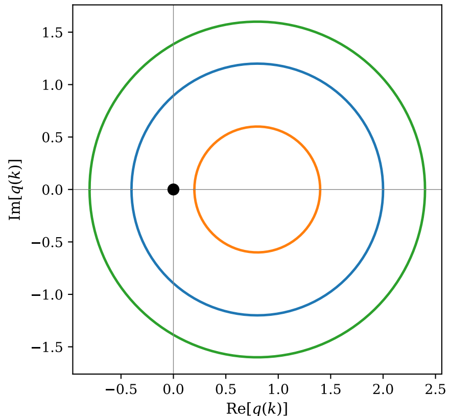
Trajectory of q(k) = t_1 + t_2 e^{-ik}
