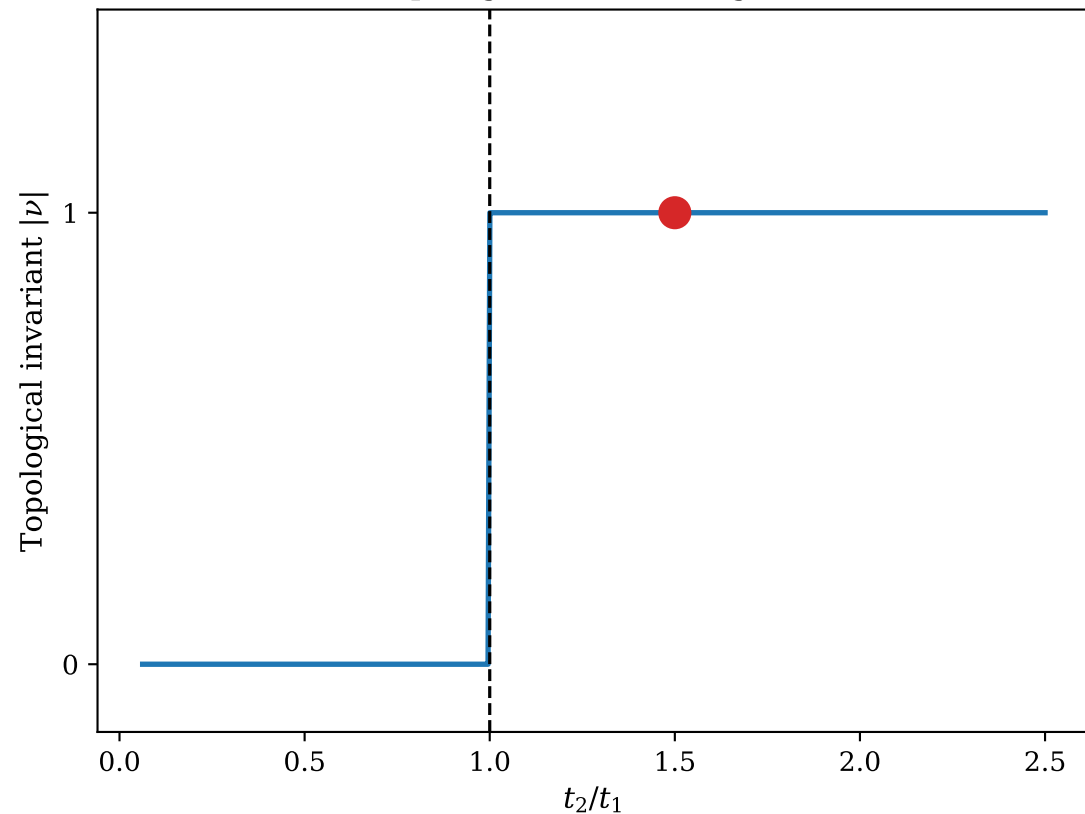
Topological Phase Diagram
