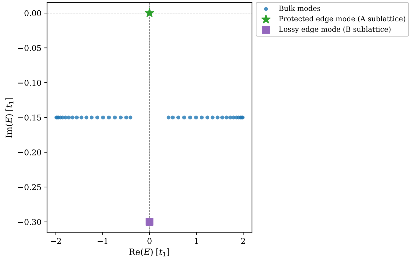
Complex Spectrum — Non-Hermitian SSH ( N = 20 )
