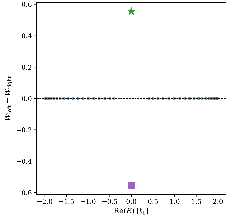
Boundary bias (biorthogonal)
