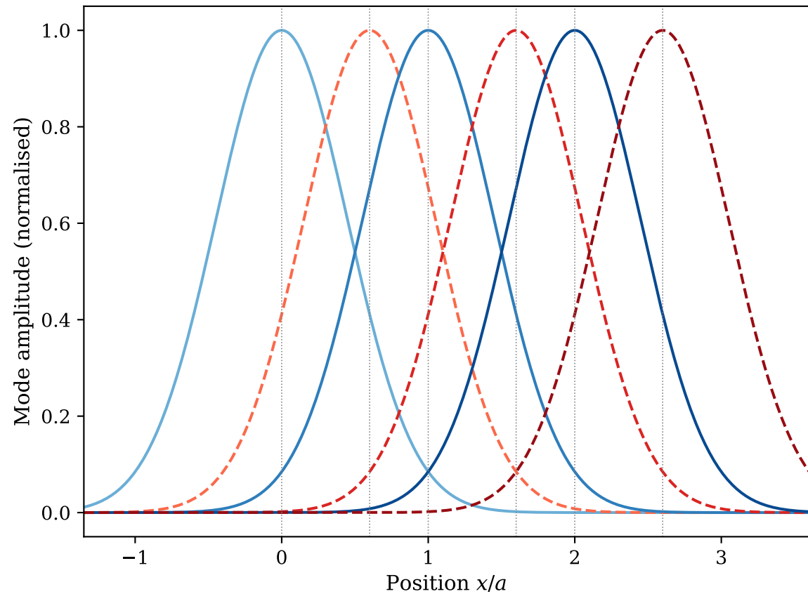
Localised Gaussian Mode Profiles
