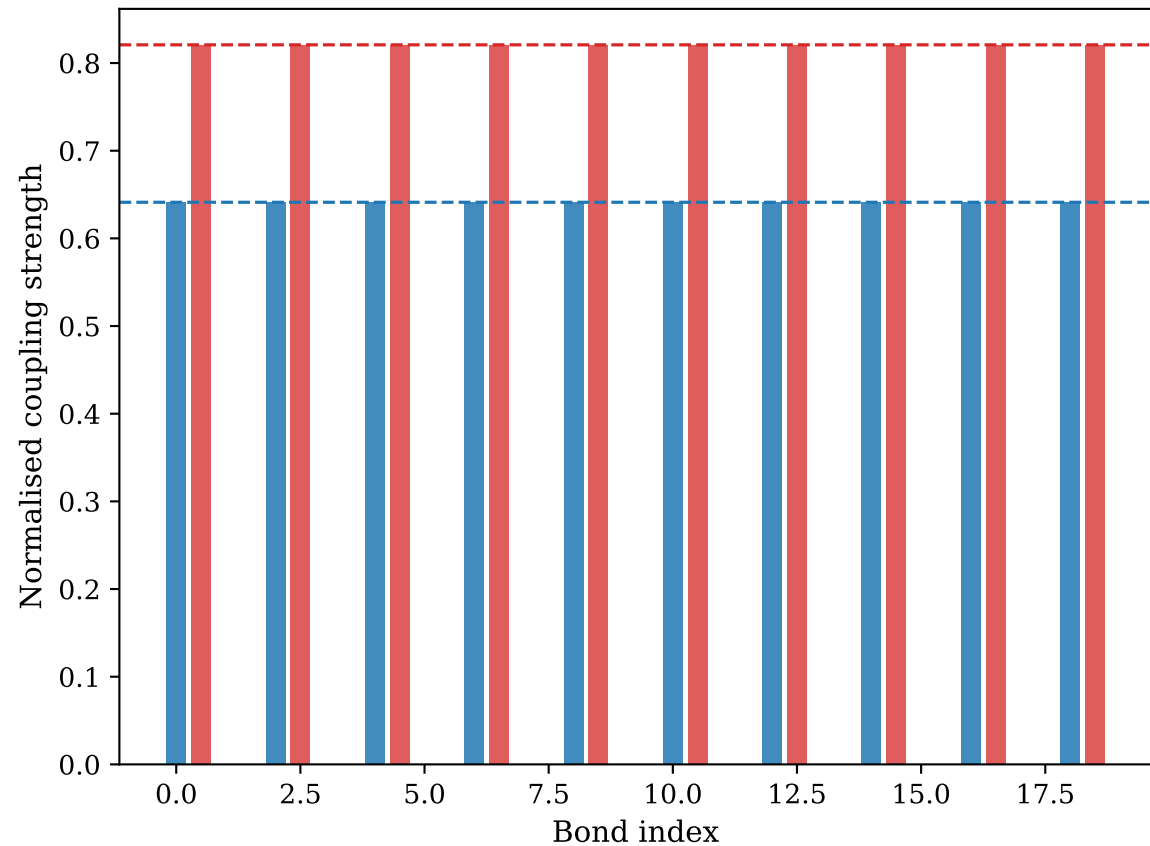
SSH Coupling Structure ( t_2/t_1 = 1.280 )
