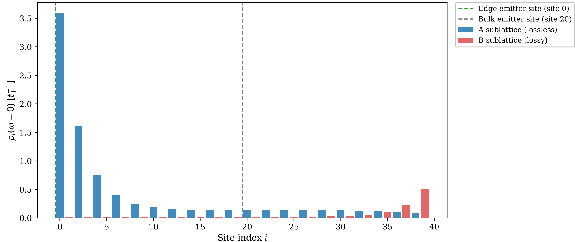
Spatial Map of LDOS at \omega = 0
