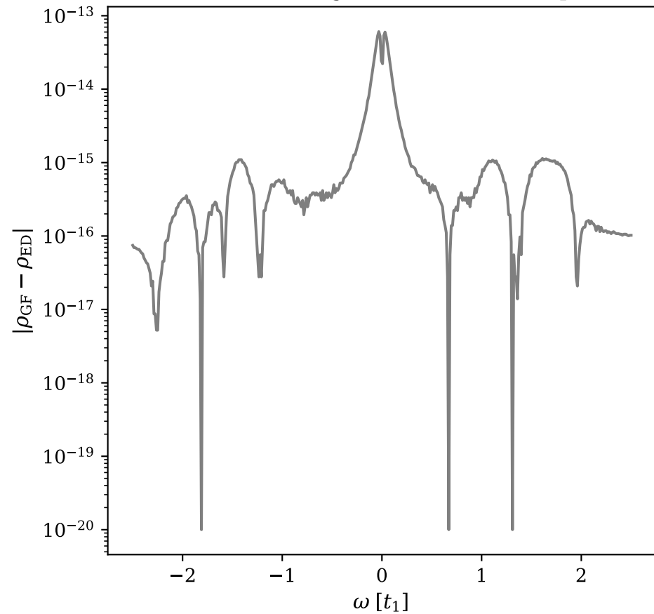
Pointwise Absolute Agreement (machine precision)
