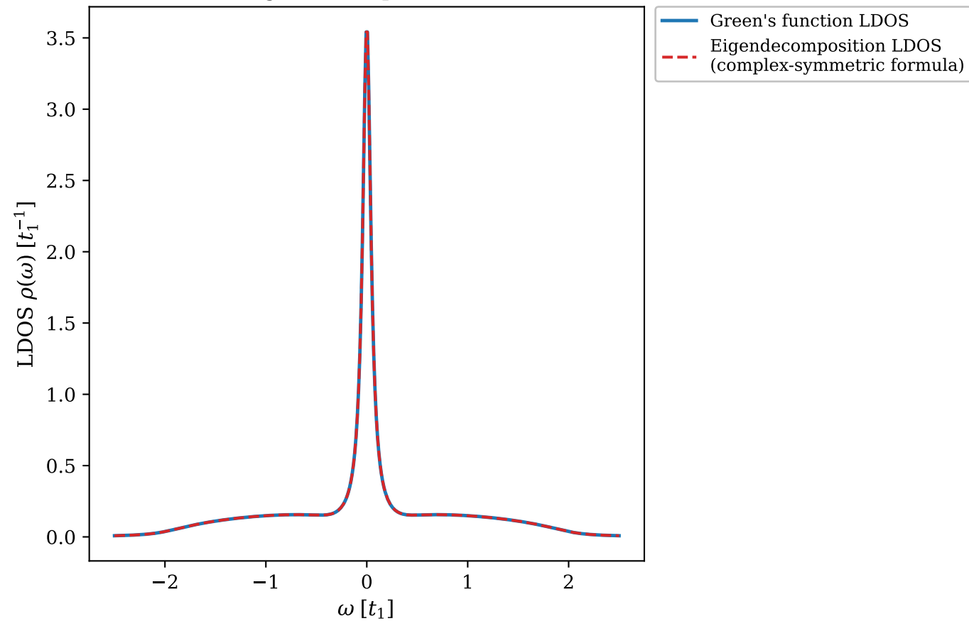
GF vs. Eigendecomposition — site 0
