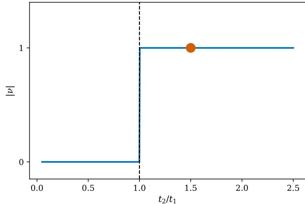
Topological invariant
