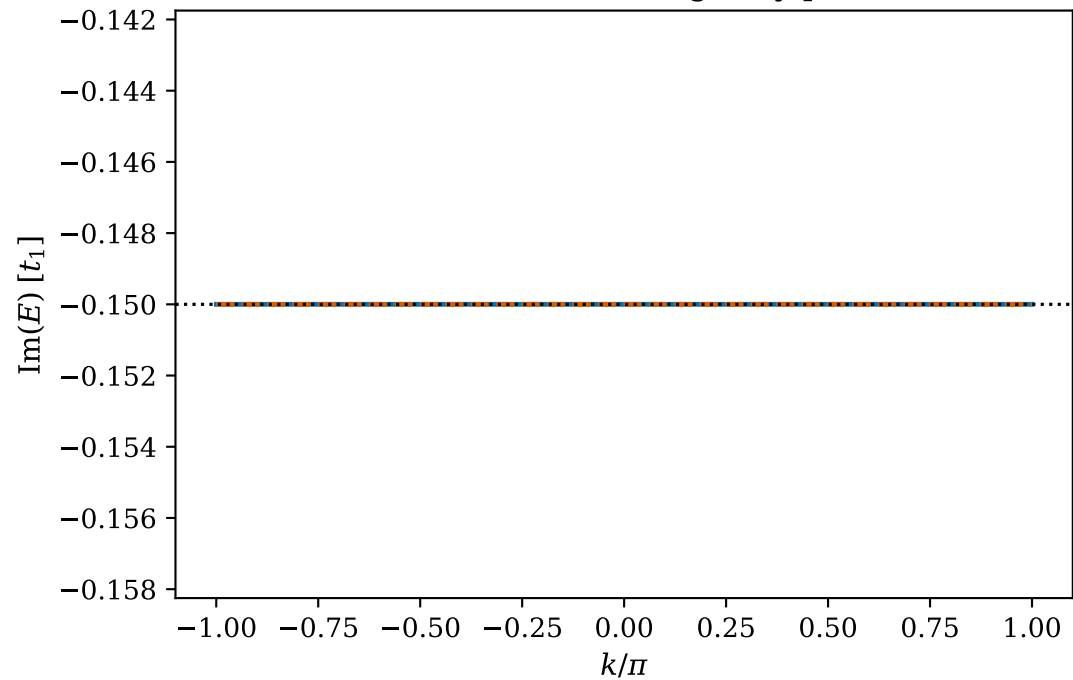
Bloch bands — imaginary part
