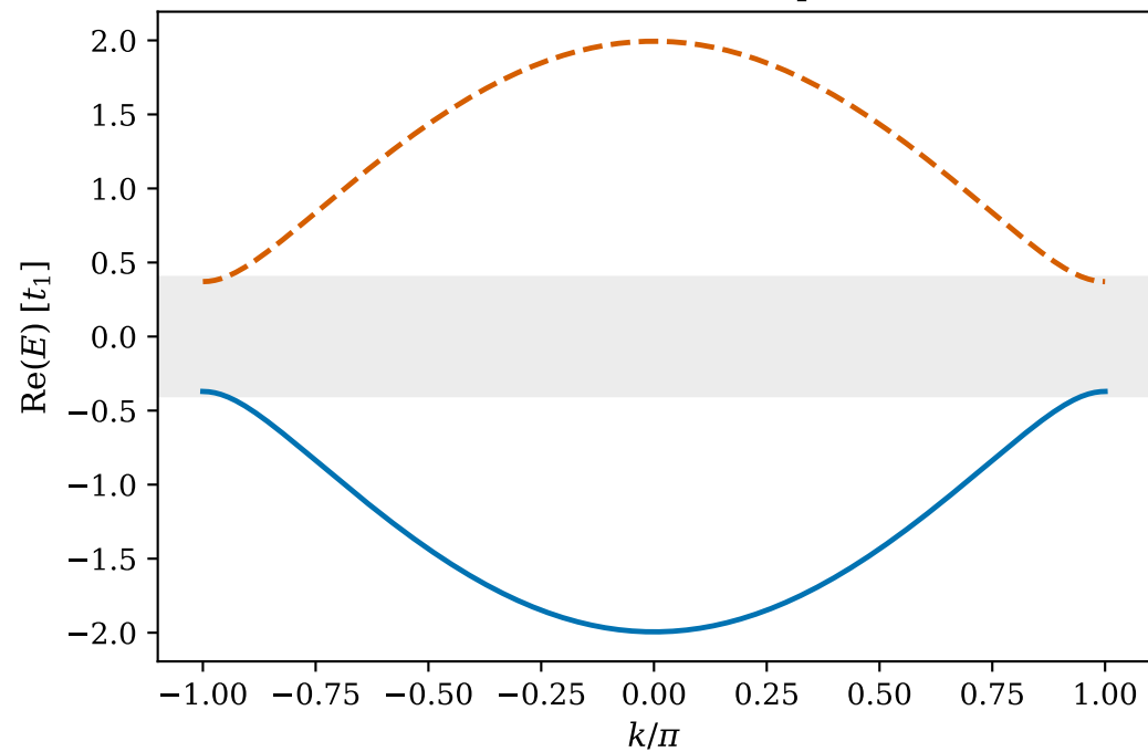
Bloch bands — real part
