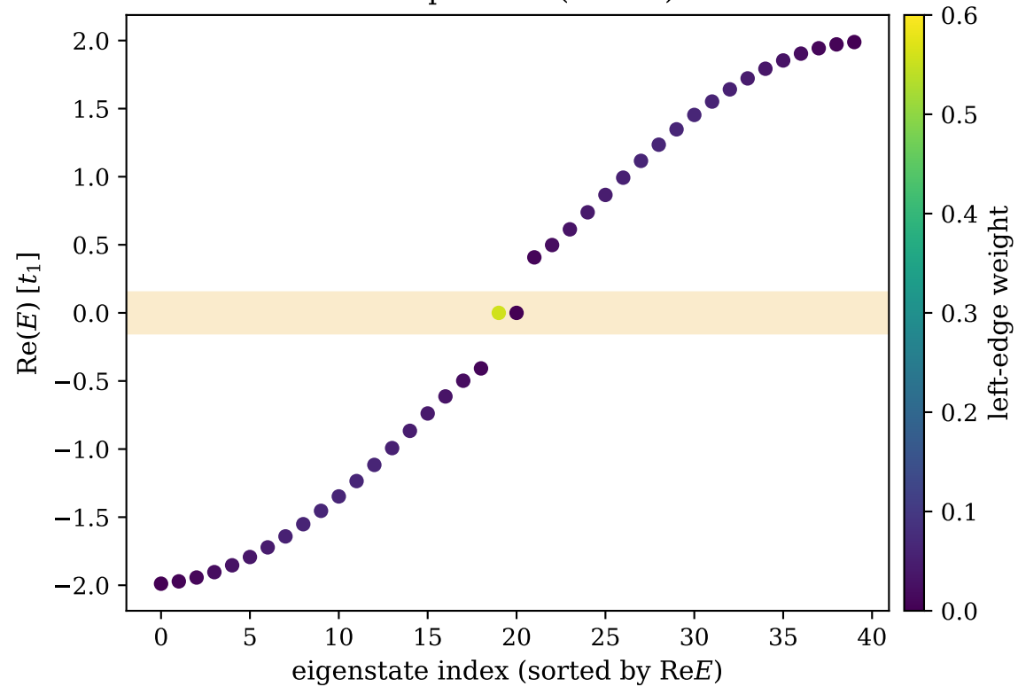
OBC spectrum ( N = 20 )
