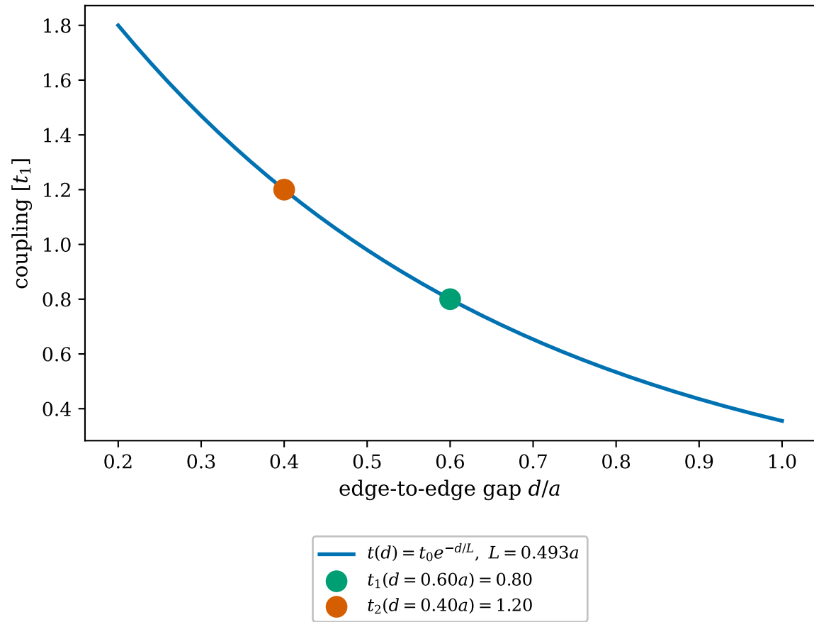
Self-consistent CMT mapping ( t_2/t_1 = 1.50 )
