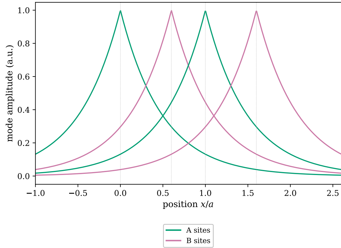
Evanescent modes \sim e^{-|x-x_0|/L}
