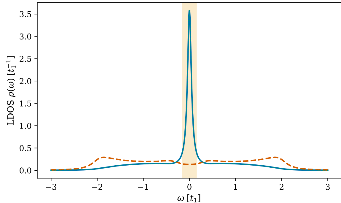
Edge vs bulk LDOS ( \eta = 0.05 t_1 )
