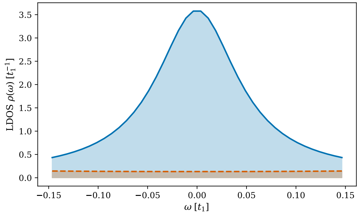
Gap region — \varepsilon = 11.2 \times (at \eta = 0.05 t_1 )
