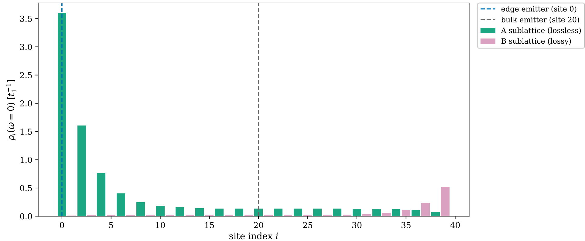
Spatial LDOS map at \omega = 0
