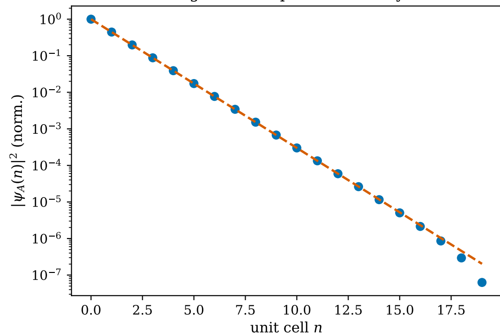
Edge-mode exponential decay
