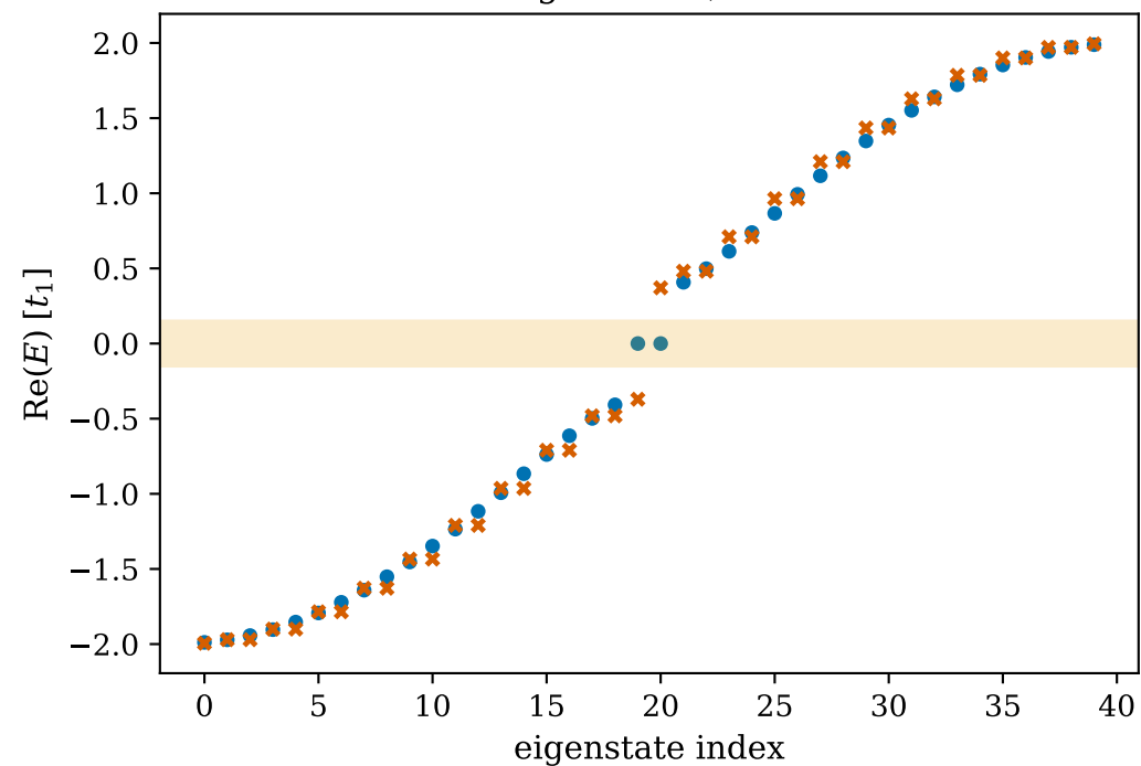
OBC has edge modes; PBC does not
