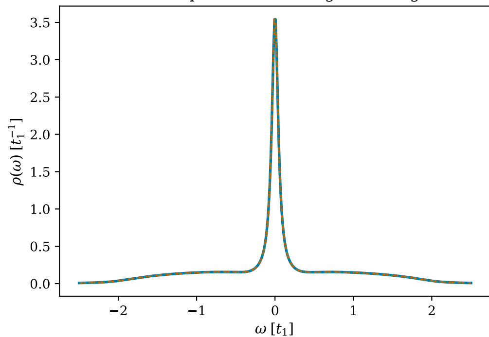
Three independent LDOS algorithms agree
