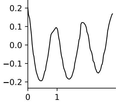
X TL ( \hat{\sigma} = 0 )
