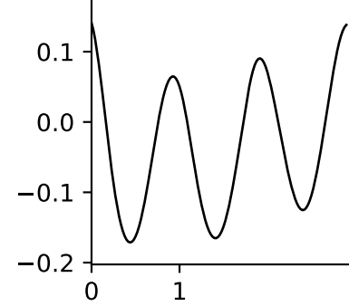
X TL ( \hat{\sigma} = 0.1 )
