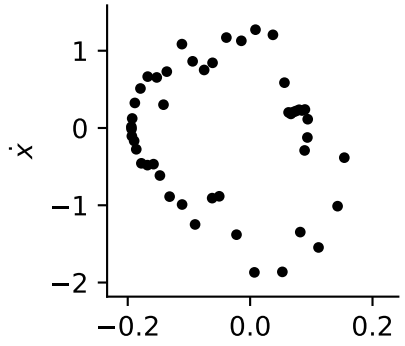
X TL (Raw 48pts)
