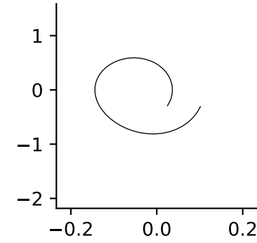
X TL ( \hat{\sigma} = 0.15 )
