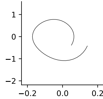
X TL ( \hat{\sigma} = 0.1 )
