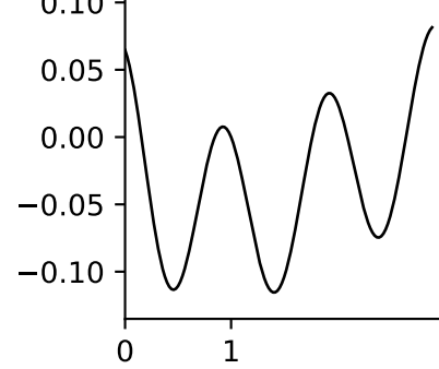
X TL ( \hat{\sigma} = 0.2 )
