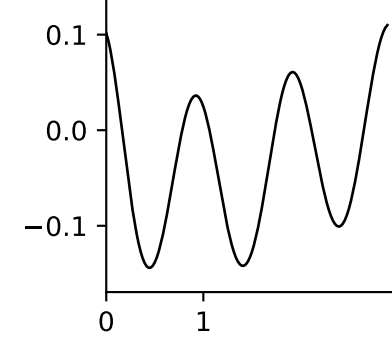
X TL ( \hat{\sigma} = 0.15 )
