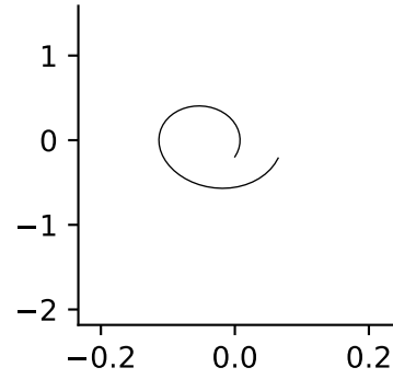
X TL ( \hat{\sigma} = 0.2 )
