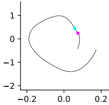
X TL ( \hat{\sigma} = 0.05 )
