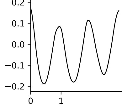
X TL ( \hat{\sigma} = 0.05 )
