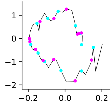
X TL ( \hat{\sigma} = 0 )
