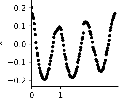
X TL (Raw 48pts)
