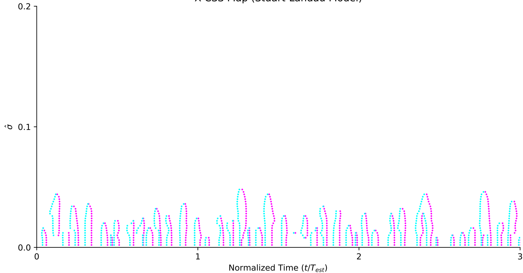
X CSS Map (Stuart-Landau Model)
