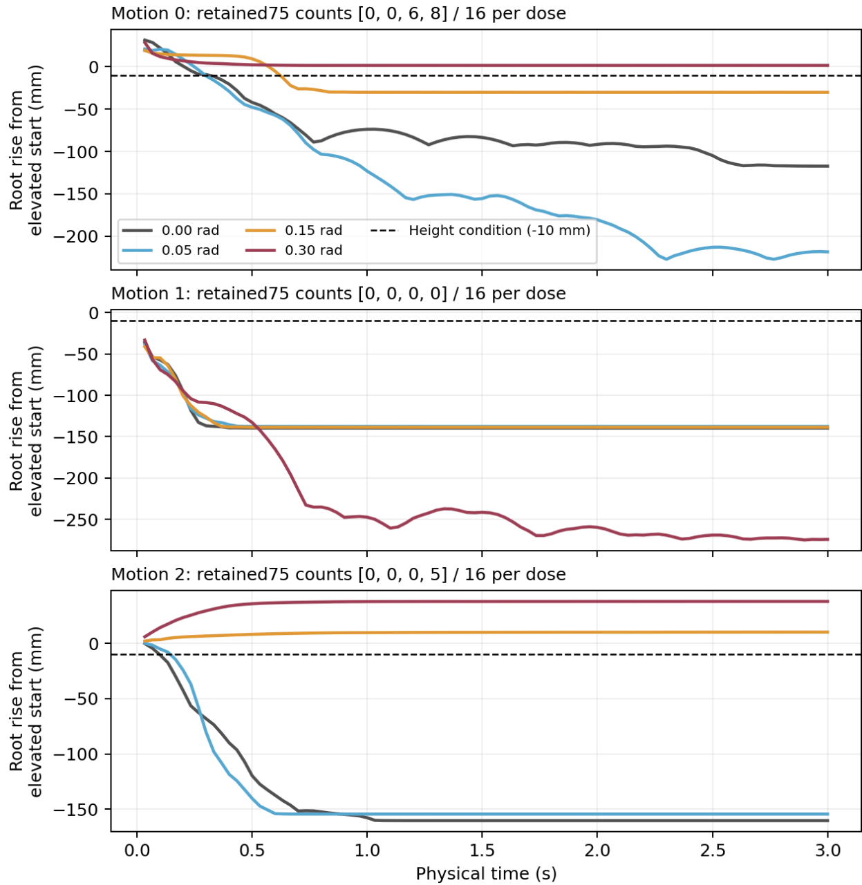
Figure 2. Physical object-root trajectories for the prospective closure screen. Each curve averages 16 trajectories per motion/dose. The dashed line is only the initial-height condition; forces, table clearance and 75 consecutive steps are additionally required. Mean height is not retained success or a policy benefit.
