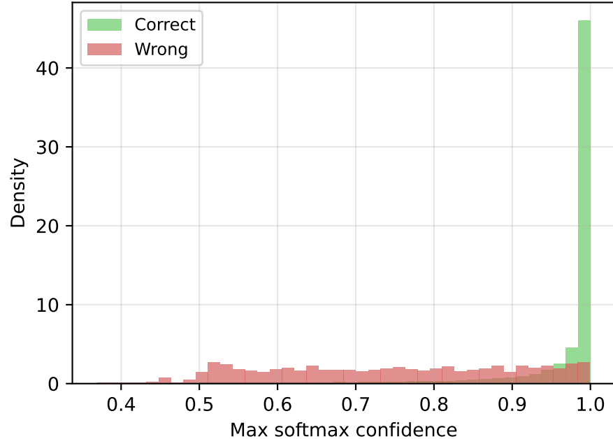
Confidence Distribution (correct vs wrong predictions)
