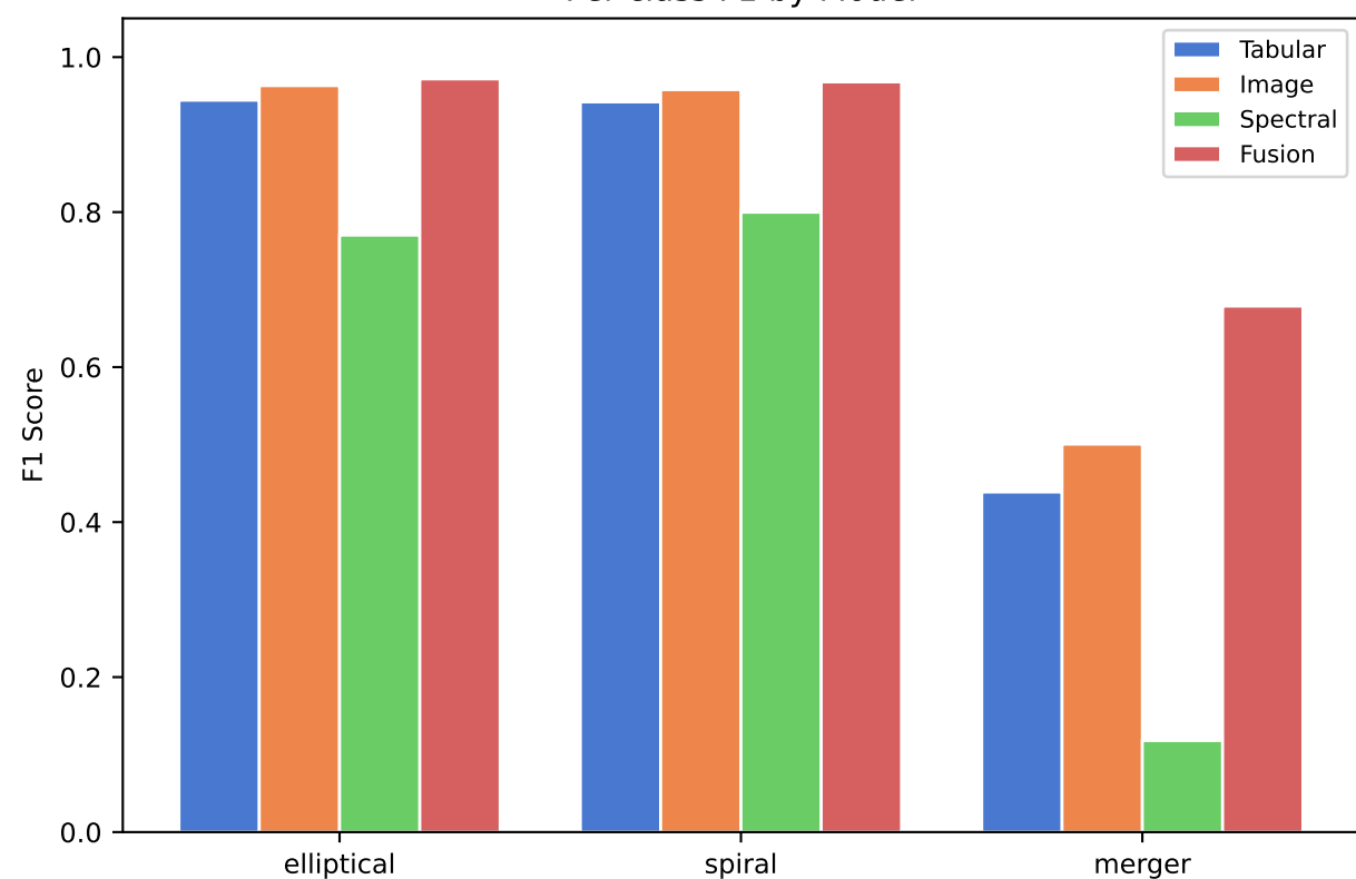
Per-class F1 by Model
