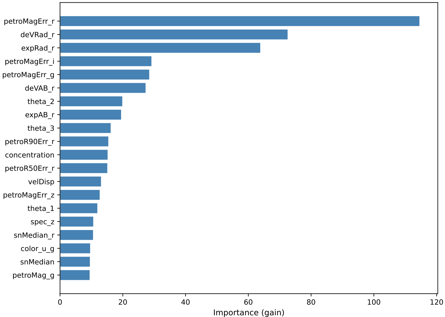
XGBoost Top-20 Feature Importances (Gain)
