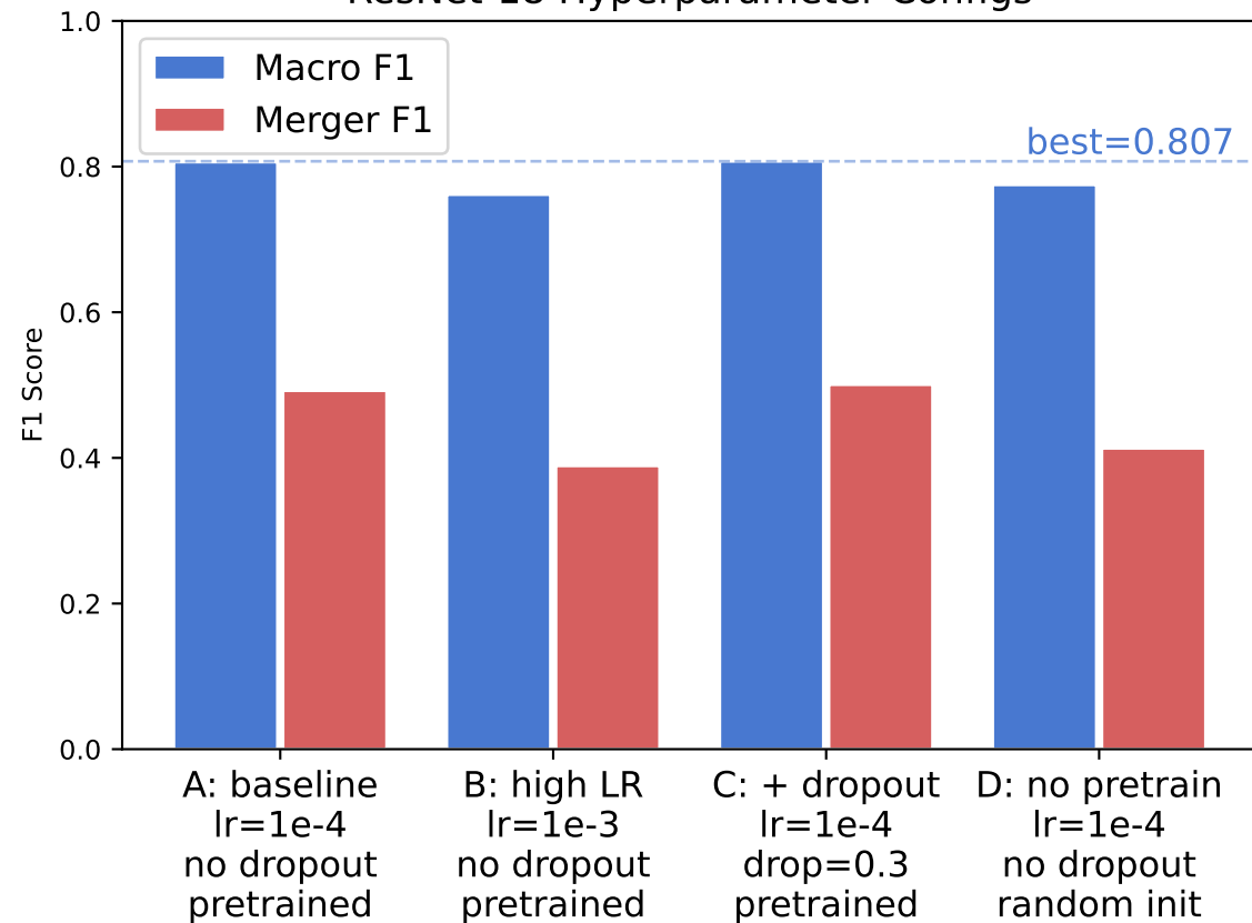
ResNet-18 Hyperparameter Configs
