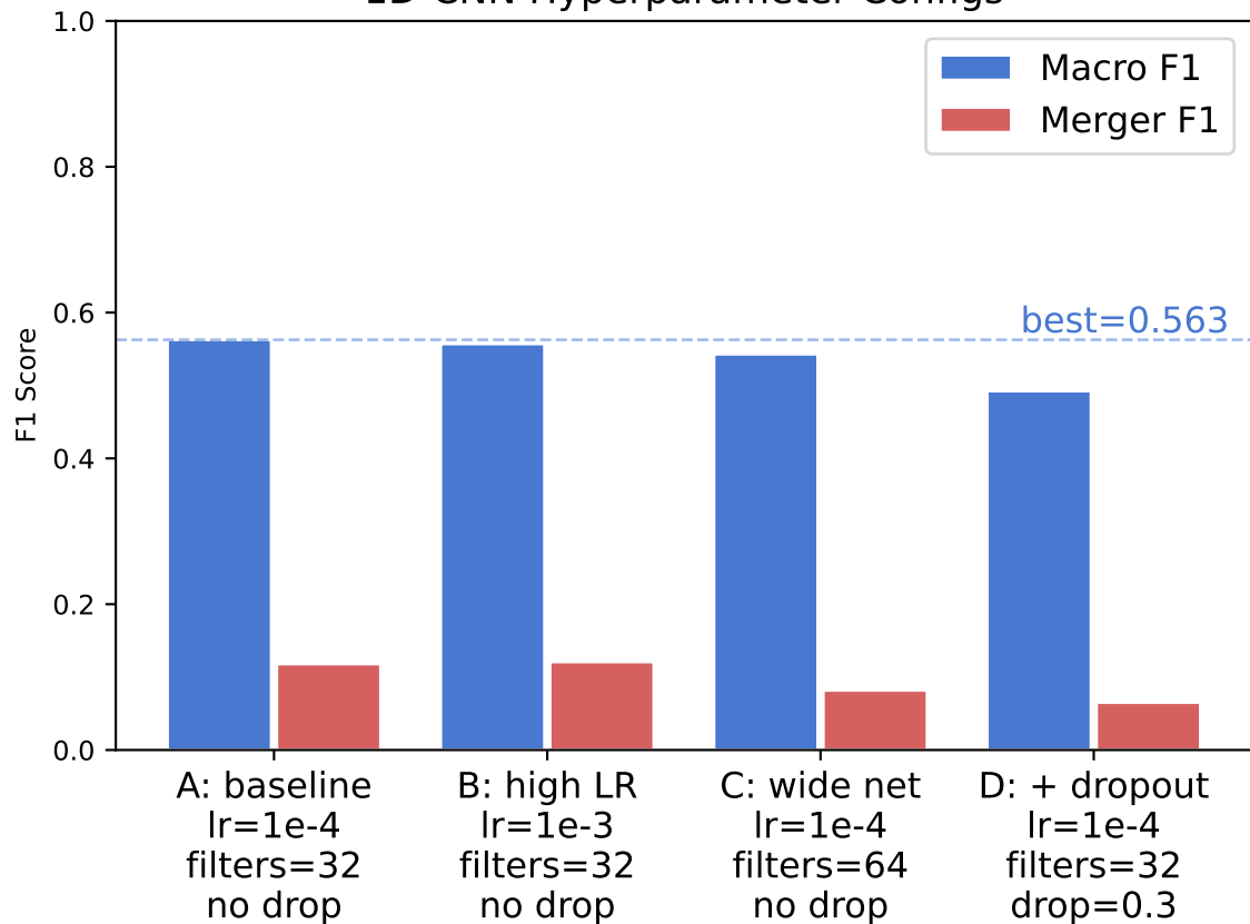
1D-CNN Hyperparameter Configs
