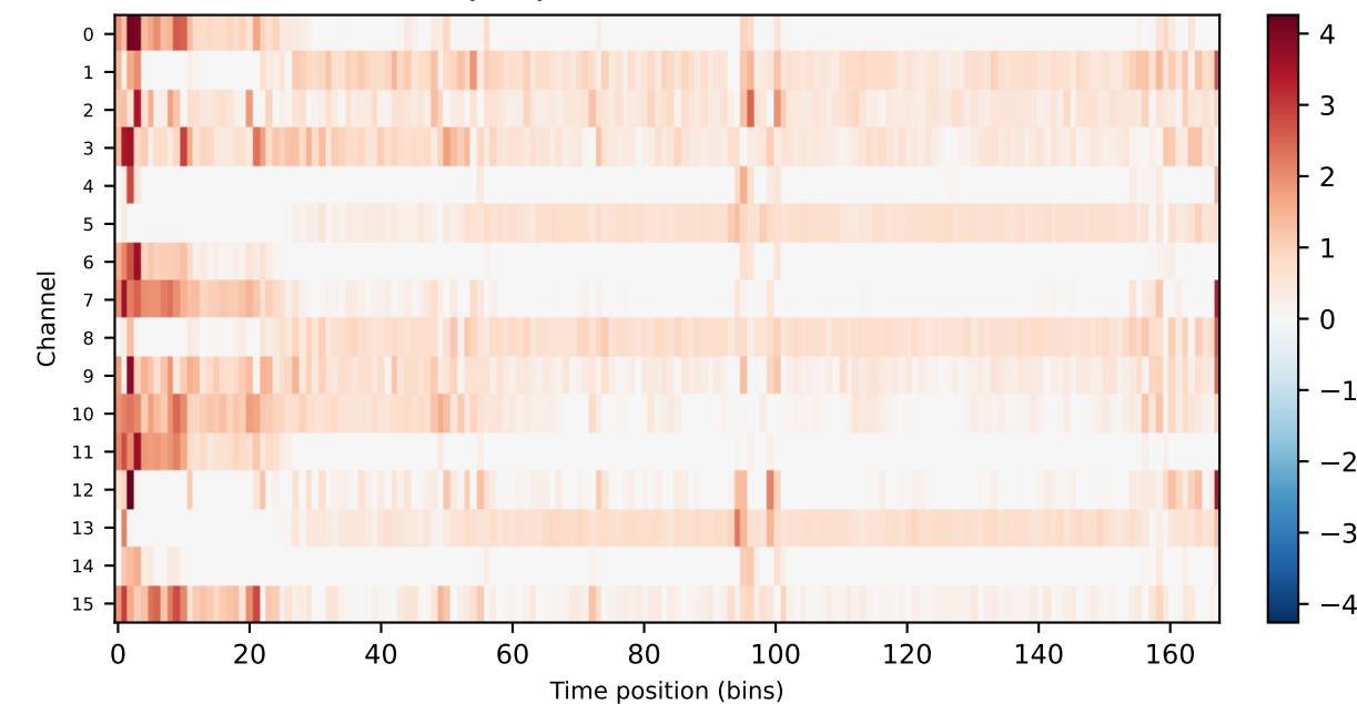
After Block 2 (64 ch x 168 bins) Conv(k=9) + BN + ReLU + MaxPool4
