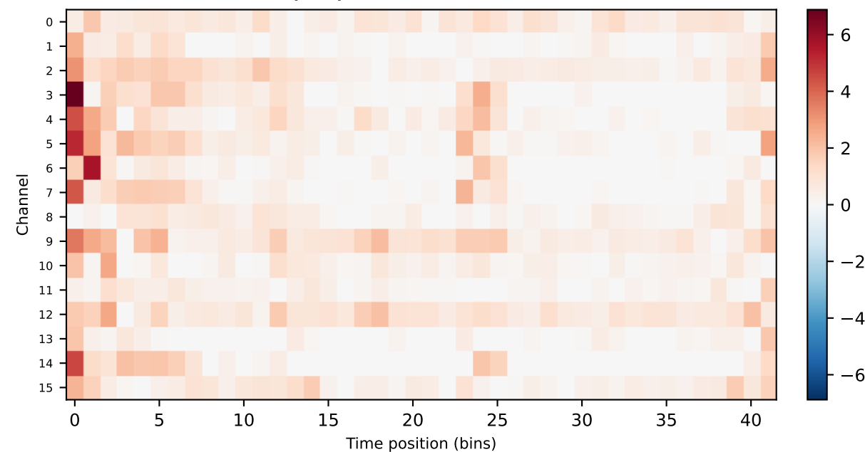
After Block 3 (128 ch x 42 bins) Conv(k=5) + BN + ReLU + MaxPool4
