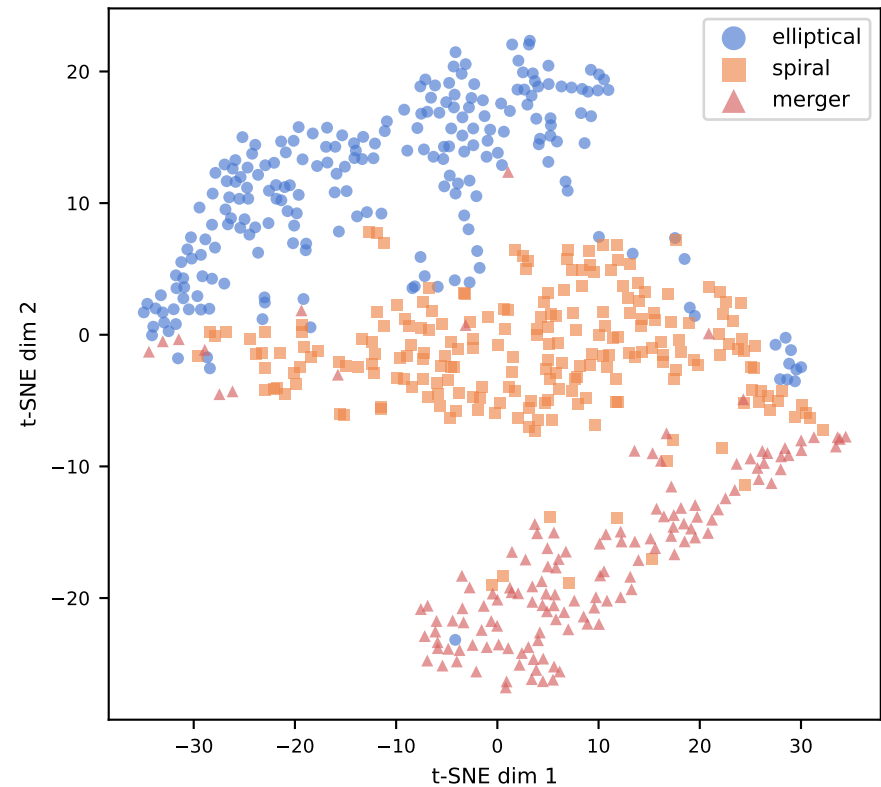
Fusion concat vector (705-d \rightarrow 2-d t-SNE)
